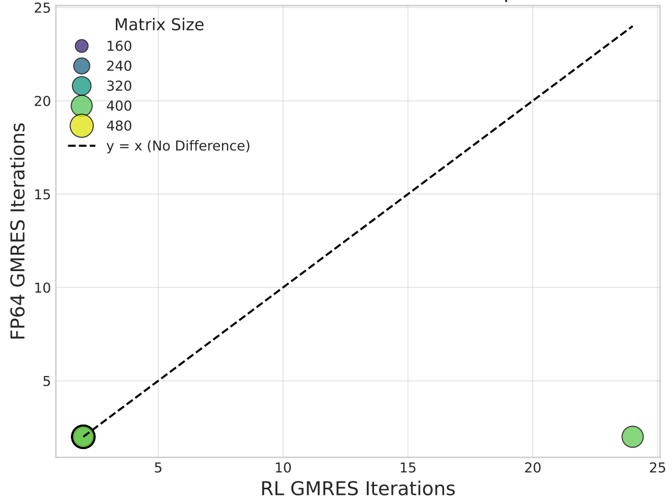
RL vs FP64 GMRES Iterations Comparison
