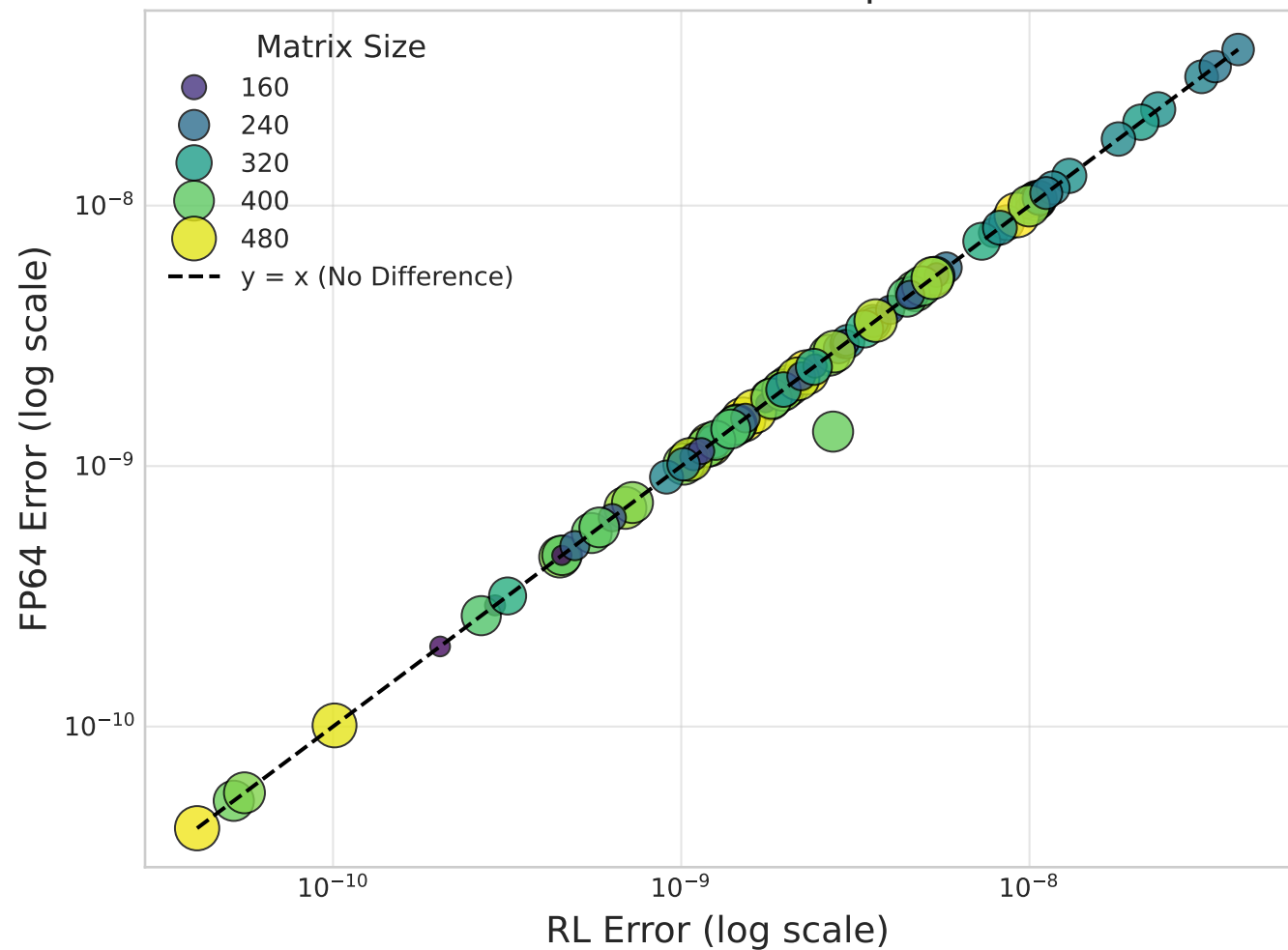
RL vs FP64 Error Comparison
