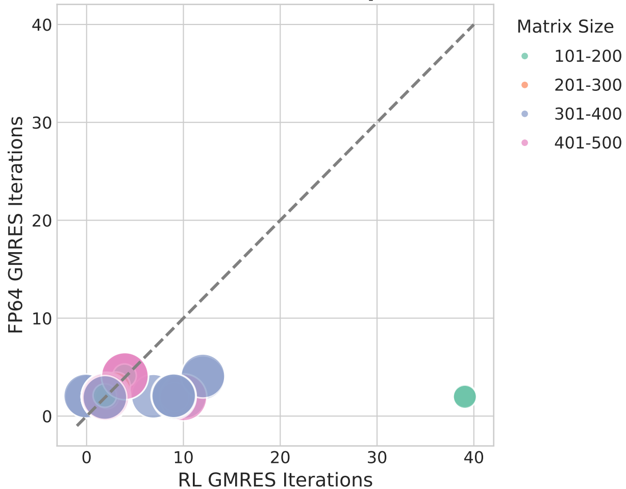
GMRES Iterations Comparison
