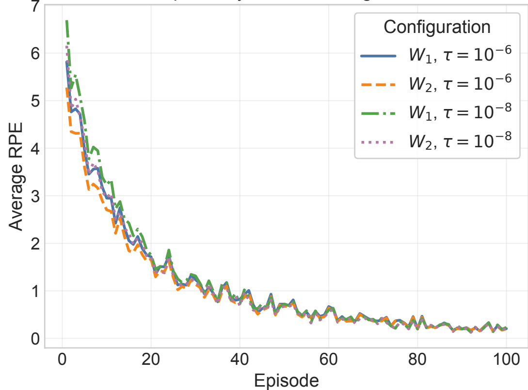
Sparse systems: training loss
