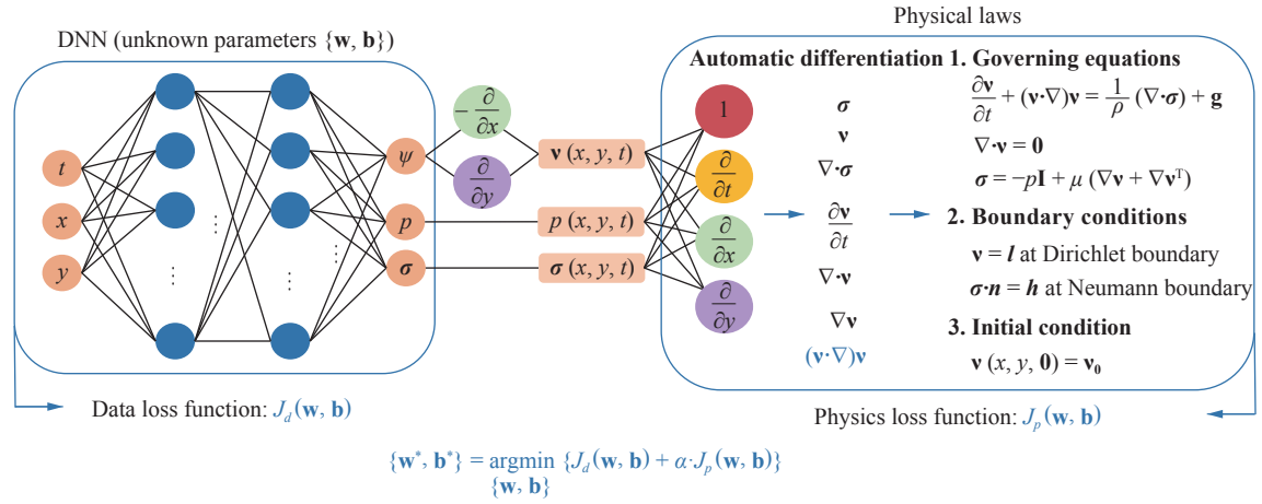
Fig. 1. Architecture of the physics-informed neural network for fluid dynamics. Note that \alpha is a user-defined weighting coefficient. w and b are weights and biases for the DNN. The constraint of initial and boundary conditions can be converted as residuals adding to the loss function based on Lagrangian multipliers. The data loss J_d is present only when data is available.
