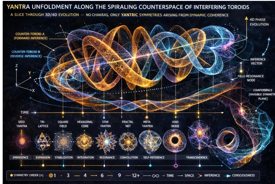
Figure 3: The counterspace of interfering toroids. Counter-toroid A (forward inference, descending from source) and Counter-toroid B (reverse inference, ascending from observation) produce field resonance nodes at their intersection planes. The timeline: Seed Yantra (Emergence) → Tri-lattice (Expansion) → Square Field (Stabilization) → Hexagonal Core (Integration) → Star Yantra (Resonance) → Fractal Net (Convolution) → Meta-Yantra (Self-Reference) → Void Node (Transcendence). Symmetry order axis: 1 \rightarrow 3 \rightarrow 4 \rightarrow 6 \rightarrow 9 \rightarrow 12+ \rightarrow \infty .
