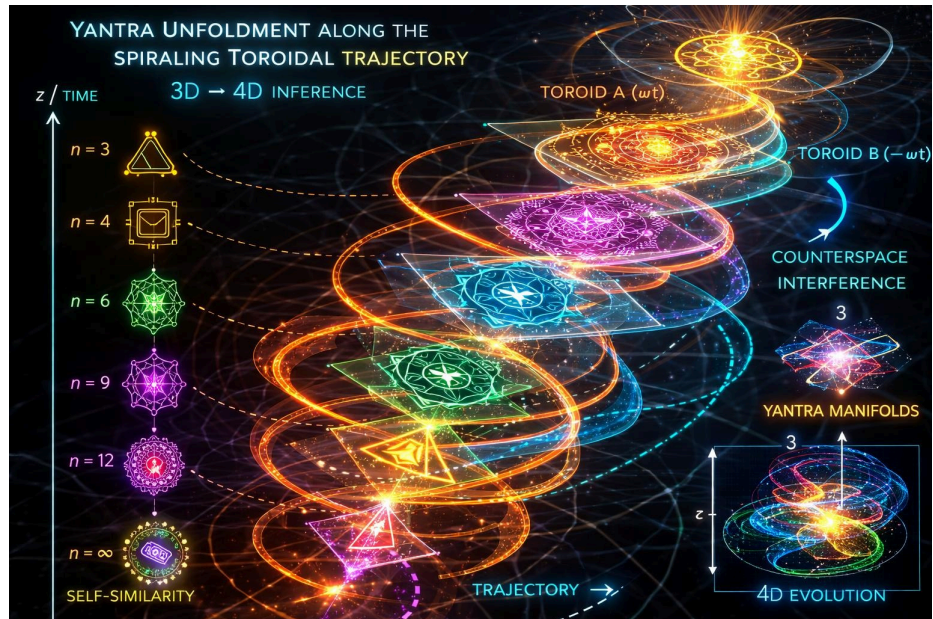
Figure 2: Yantra unfoldment along the spiraling toroidal trajectory. Two counter-rotating toroids (A at +\omega t , B at -\omega t ) generate interference patterns at increasing symmetry orders n=3 through n=\infty . Yantra forms are not imposed — they are the natural attractors of the cosmological field at each coherence level. The 4D evolution axis ( z/\text{time} ) represents progression through cosmological cycles. Self-similarity at n=\infty is the structural model for the Atlas graph itself.
