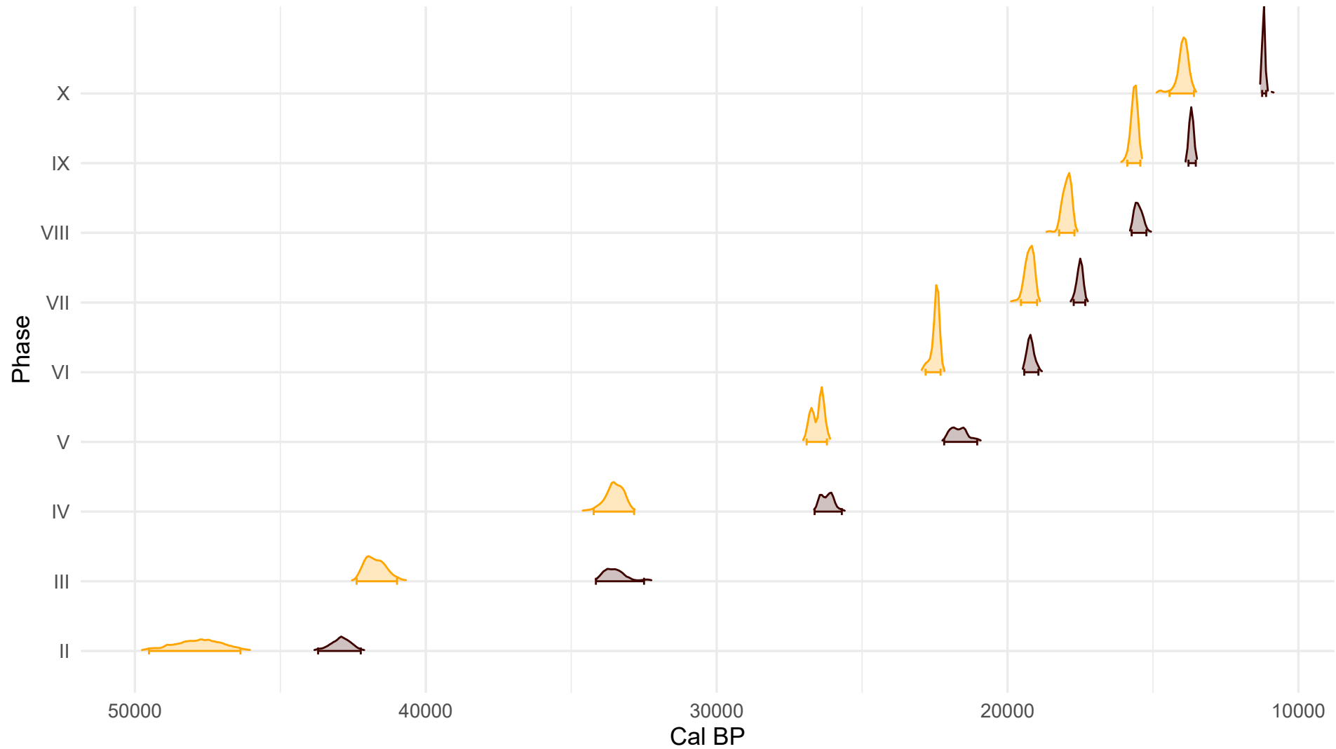
Phase posterior densities and 95% HPD intervals – Phase II–X
