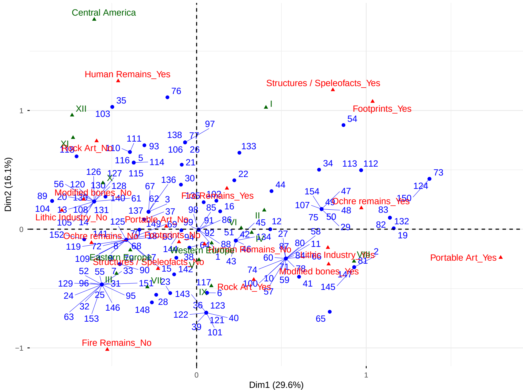
MCA – Biplot
