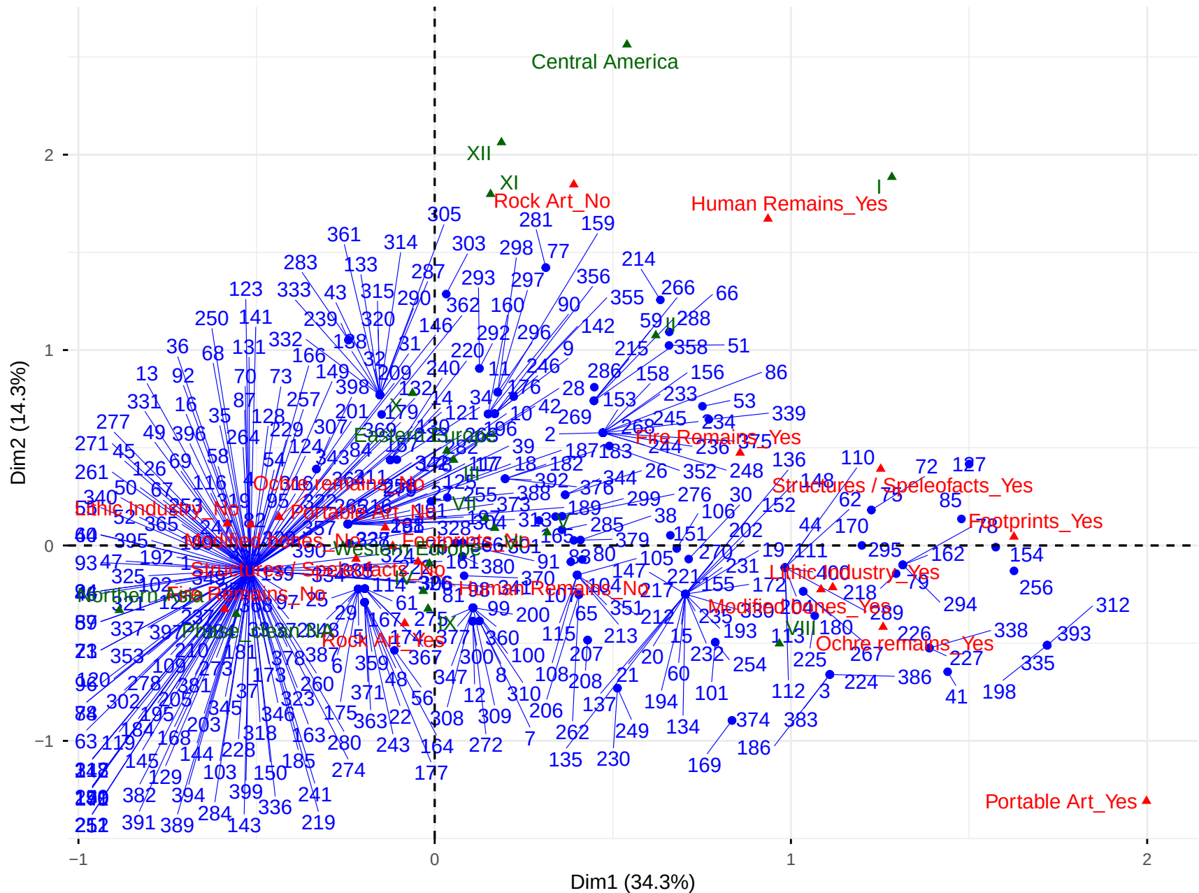
MCA – Biplot
