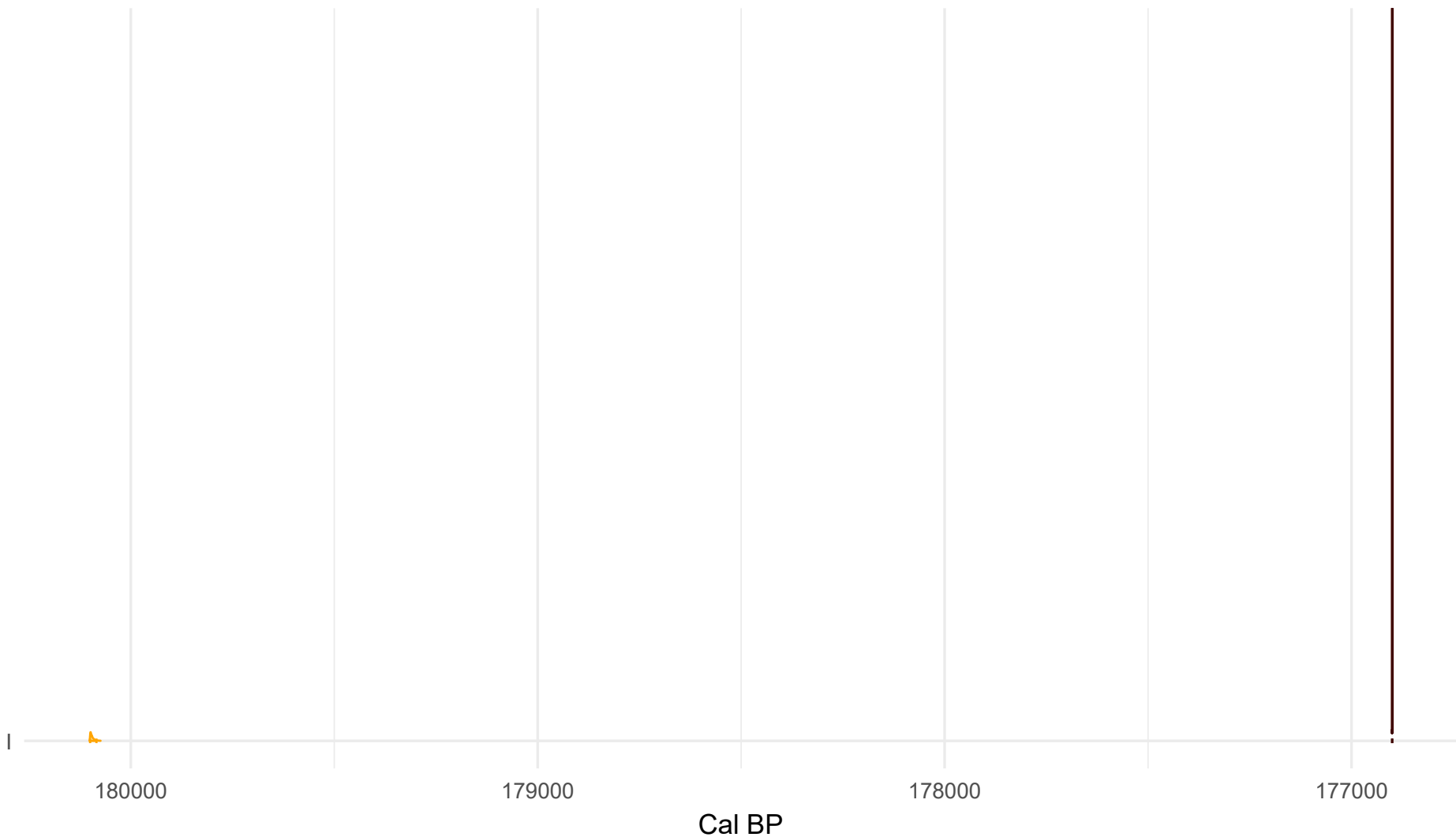
Phase posterior densities and 95% HPD intervals – Phase I
