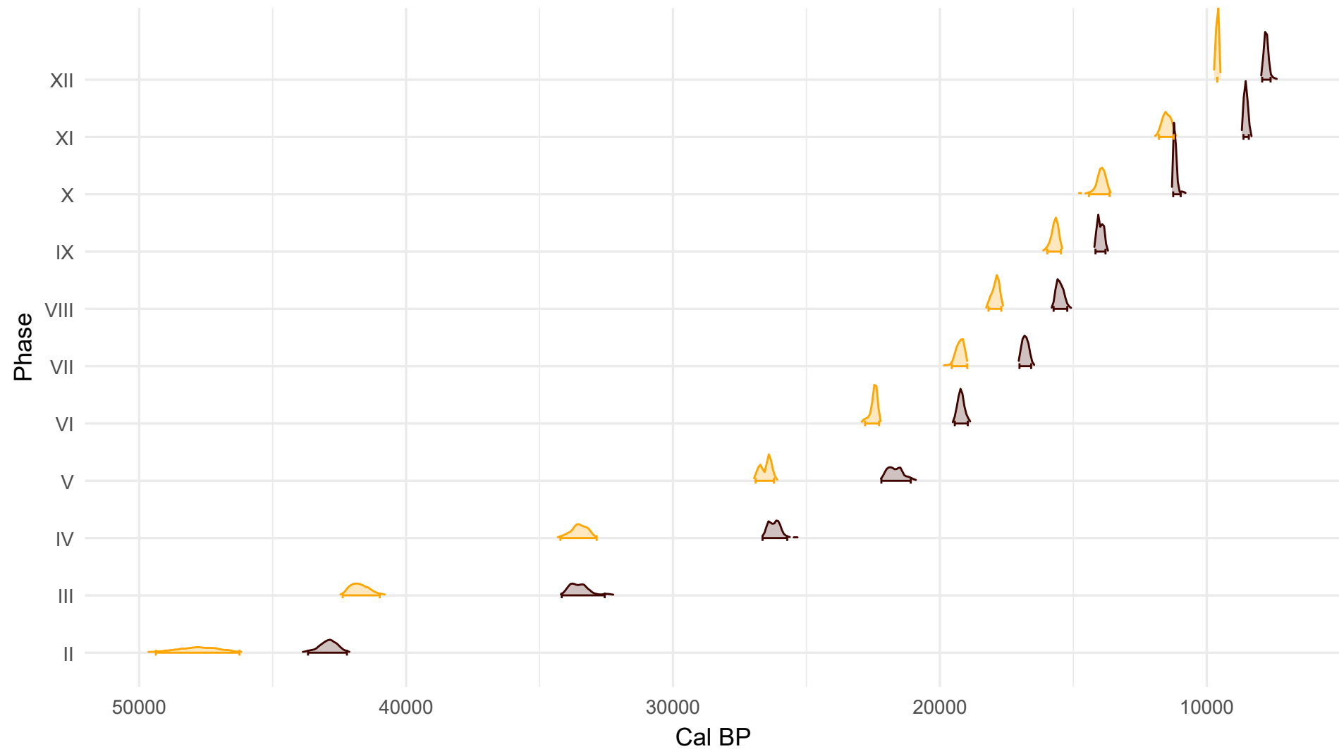
Phase posterior densities and 95% HPD intervals – Phases II–XII
