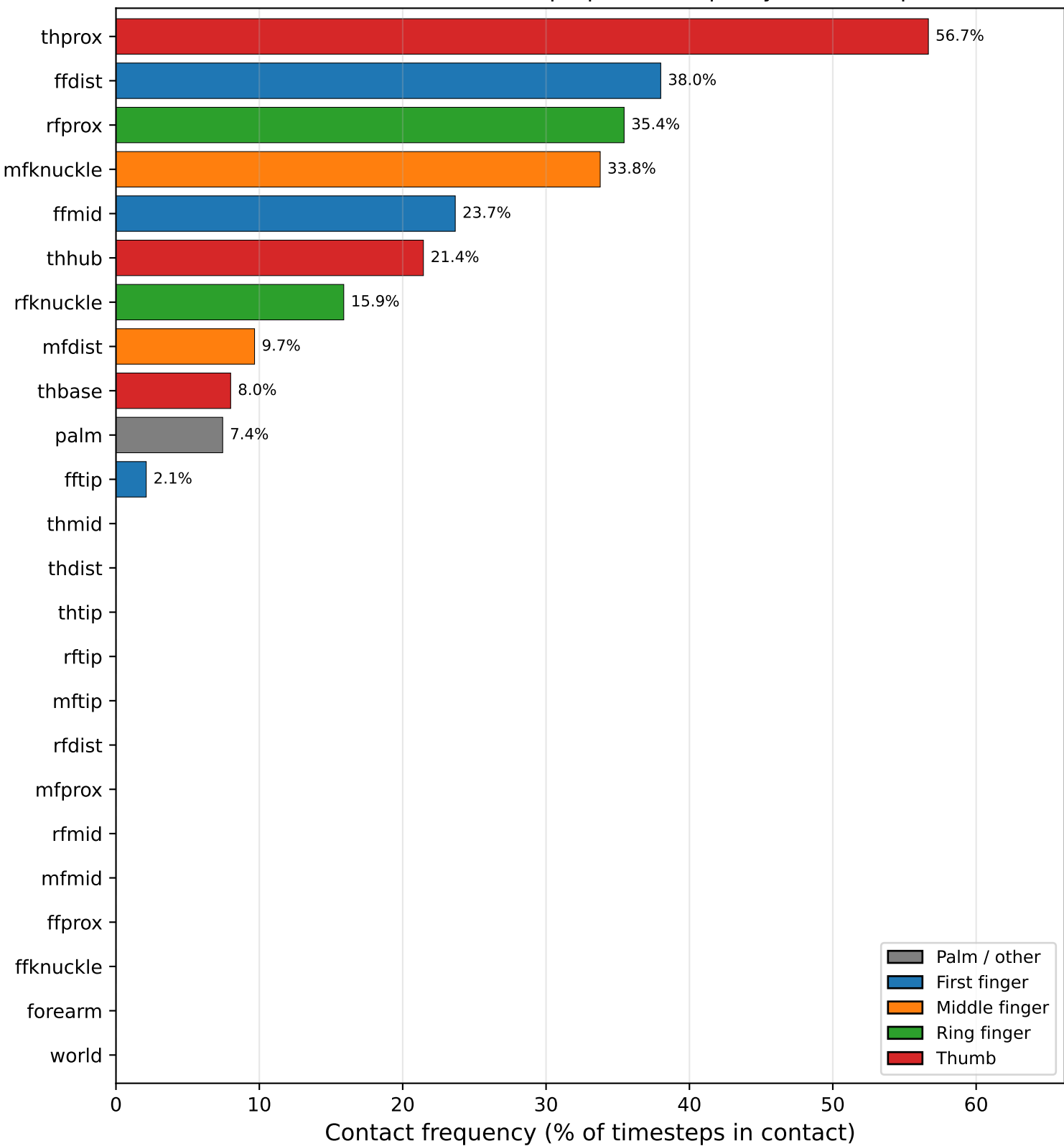
Per-link tactile activation during Baoding Shadow Hand Lite, blind (prop+tactile) policy — 900 steps
