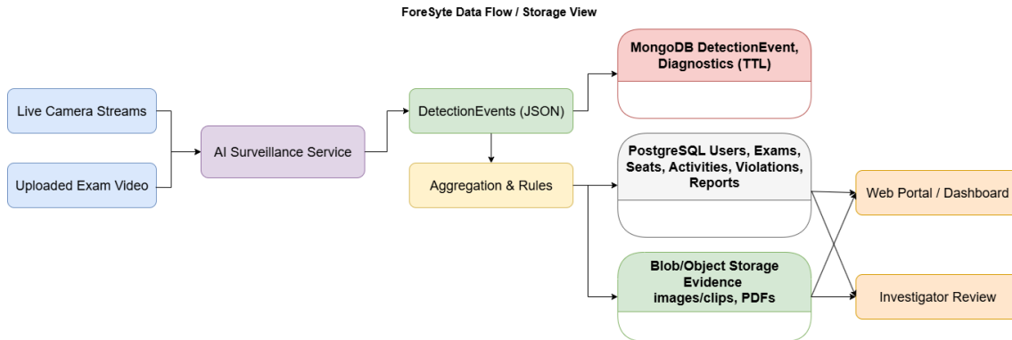
Figure 3.2: Data Flow and Storage View (PostgreSQL, MongoDB, Blob/Object Storage)
