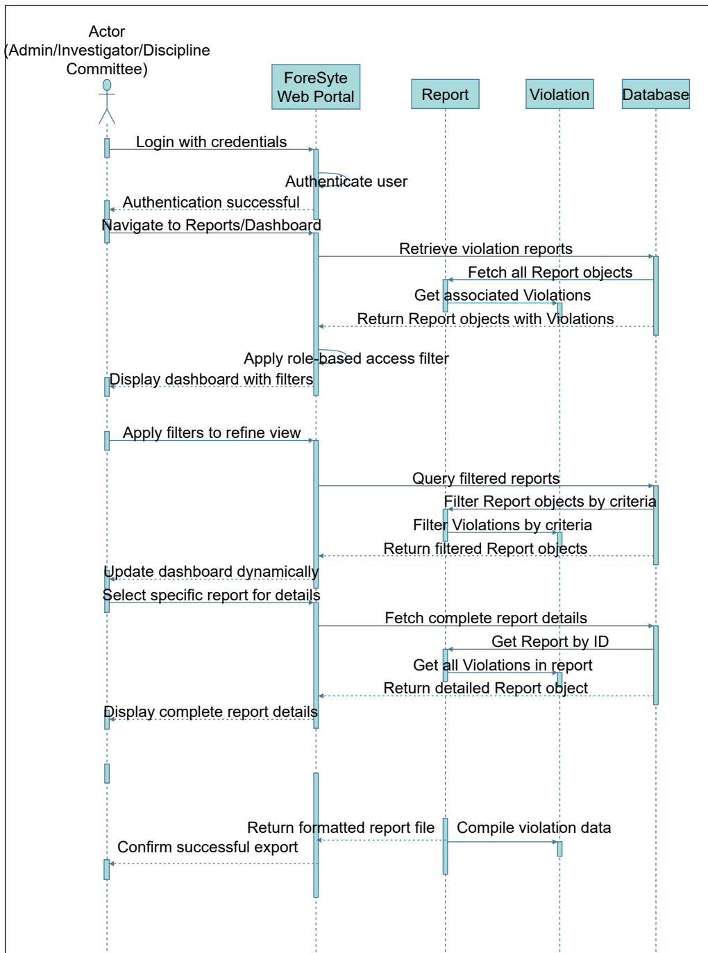
Figure 3.6: Sequence Diagram for UC-01: View and Manage Reports/Dashboard
