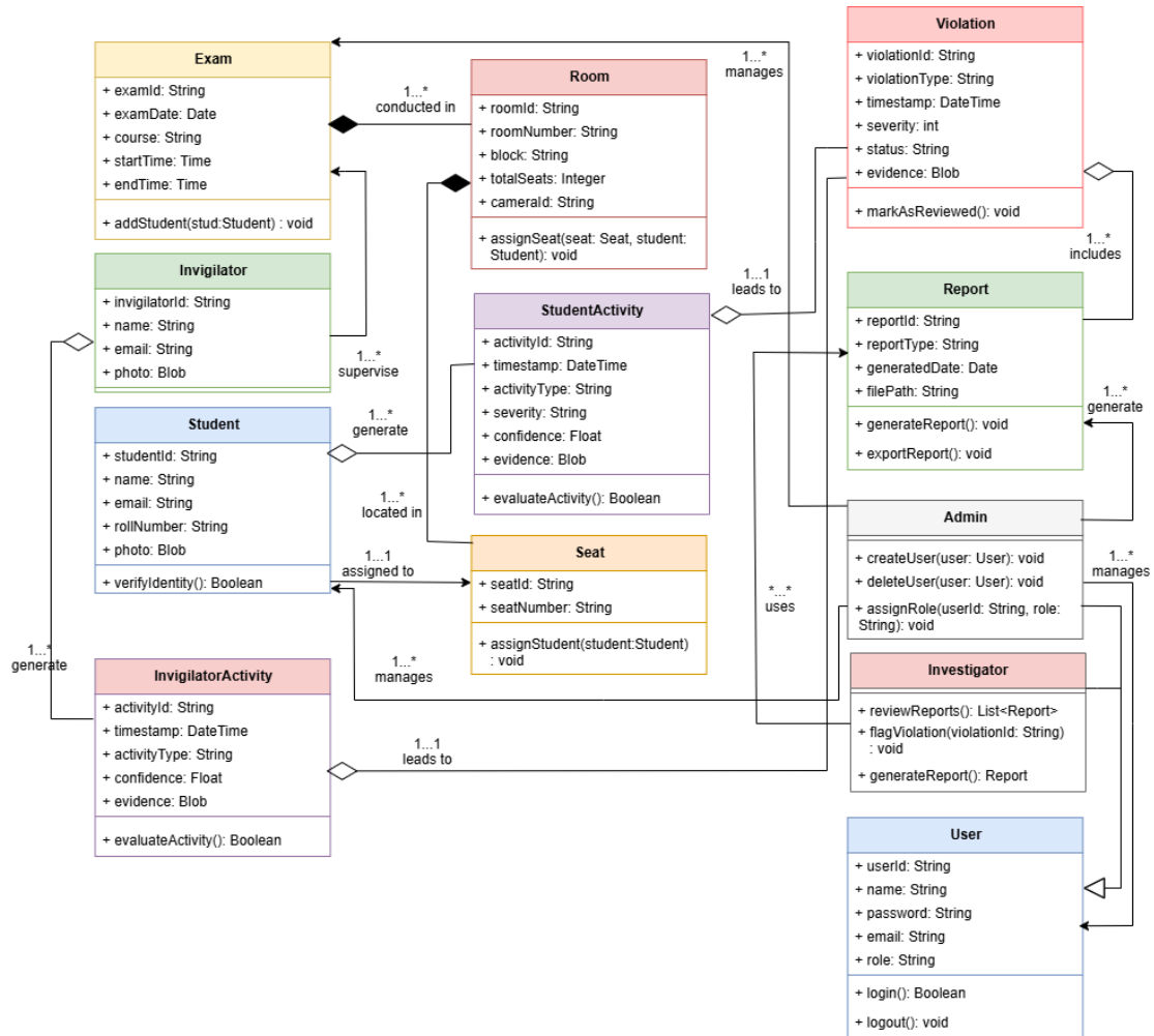
Figure 3.4: ForeSyste Class Diagram
