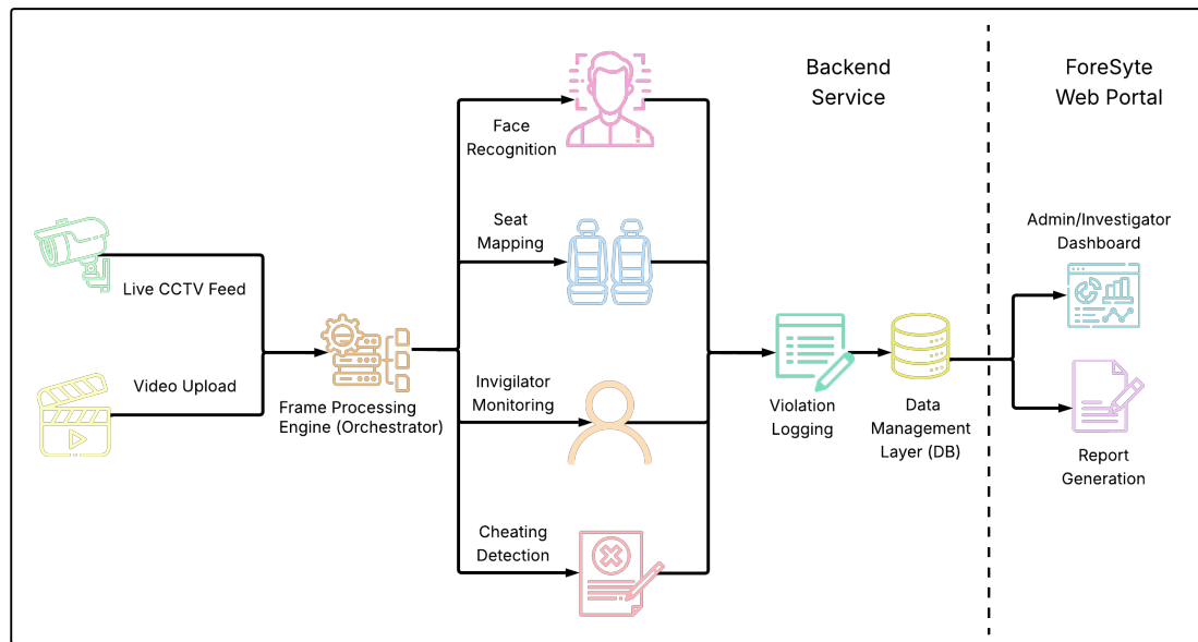
Figure 3.1: High-Level Architectural Design of the ForeSyte AI Exam Surveillance System
