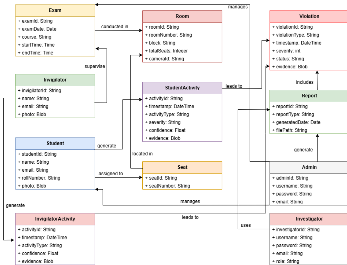
Figure 3.3: ForeSyste Domain Model Diagram
