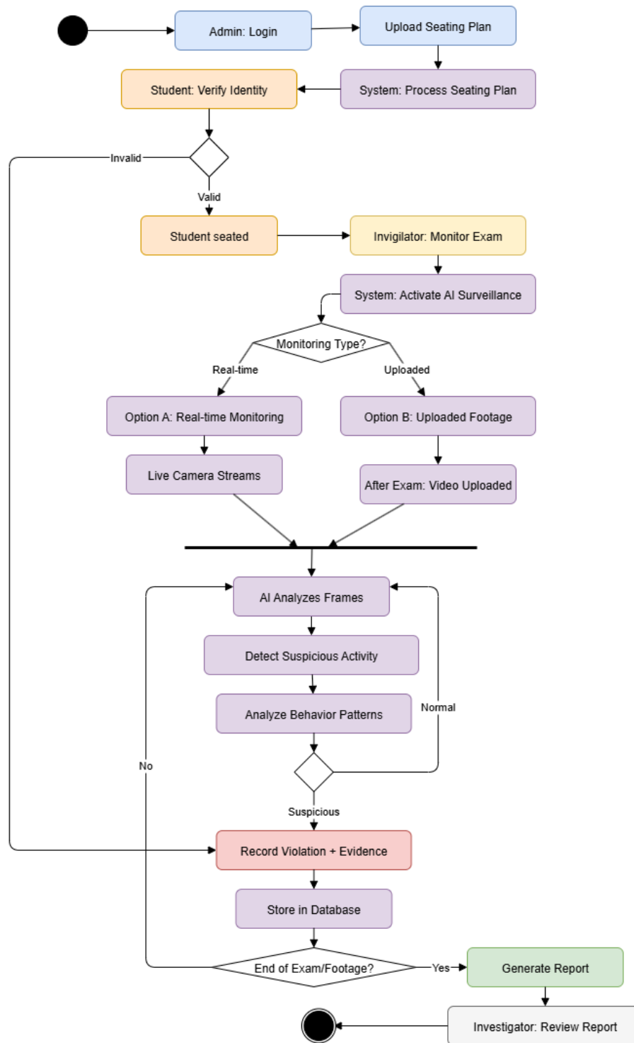
Figure 3.5: ForeSyte Activity Diagram
