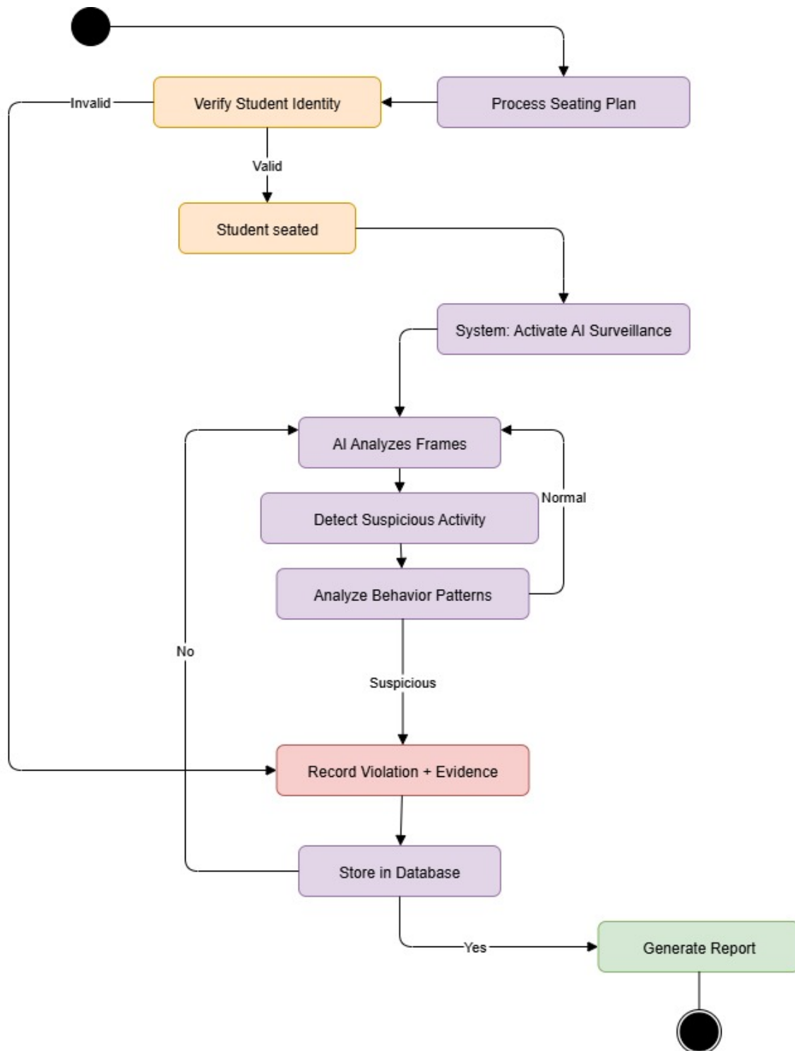
Figure 3.13: State Transition Diagram
