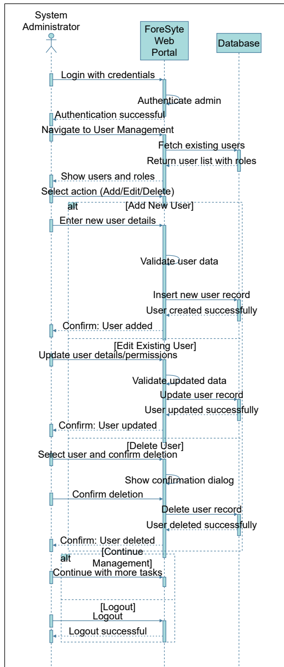
Figure 3.7: Sequence Diagram for UC-02: Manage User Profiles
