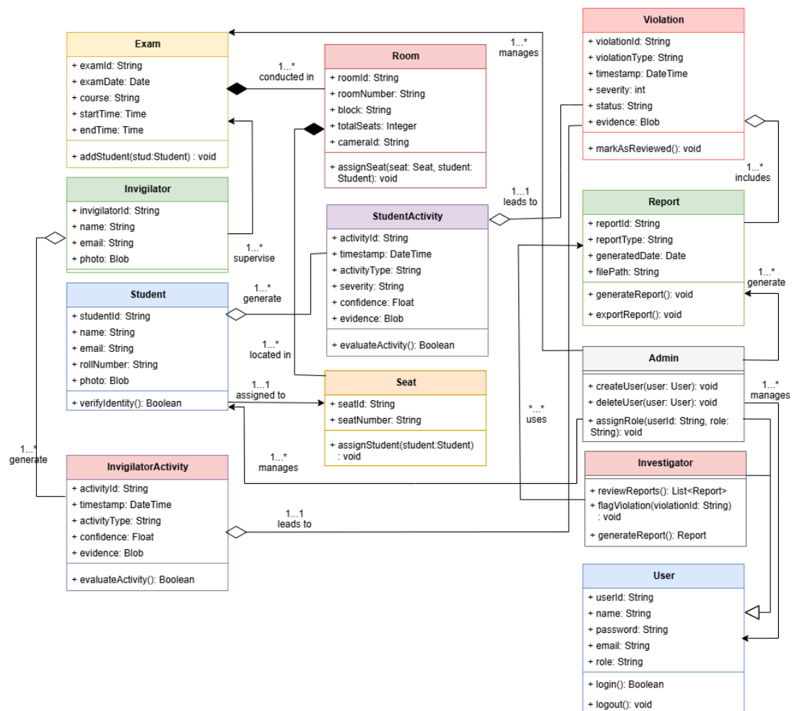
Figure 3.5: ForeSyte Class Diagram
