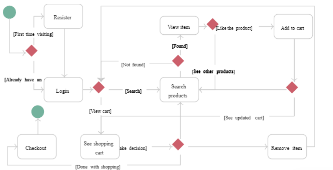
Figure A.11: State Transition Diagram For Online Shopping Application
