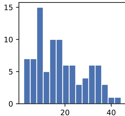
Small-world \sigma
