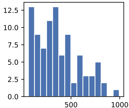
Nodes
