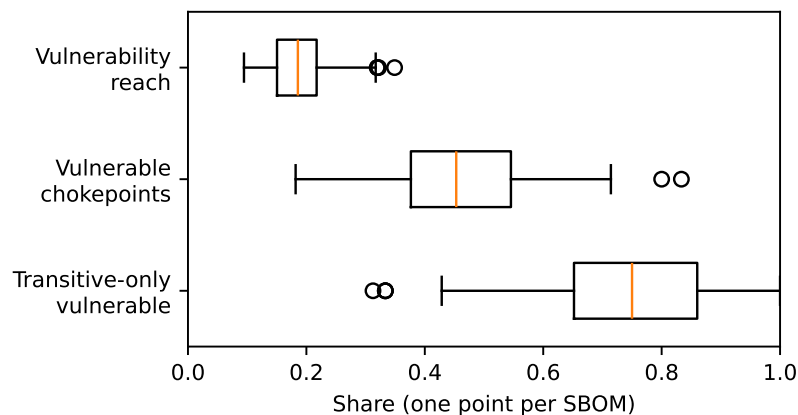
Figure 7.3: Transitive-only share of vulnerable components, share of vulnerable components that are chokepoints, and vulnerability reach, over the 90 SBOMs.
