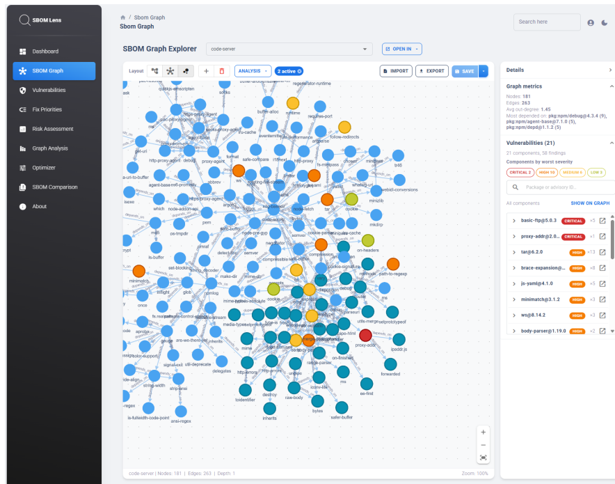
Figure 5.3: Dominated set of express in the code-server SBOM (cyan): the components reachable from the root only through express , which would lose their connection to the application if it were removed. The severity colours of the vulnerable components are also shown.
