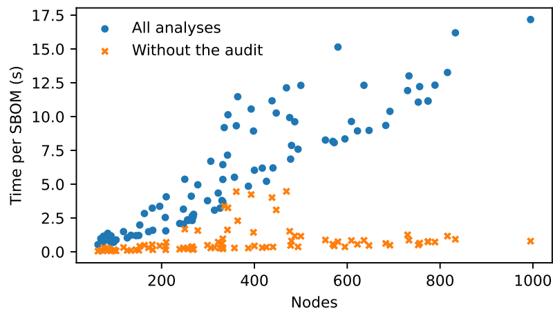
Figure 7.4: Total analysis time per SBOM against its number of nodes, with and without the audit, whose time is dominated by queries to the npm registry.
