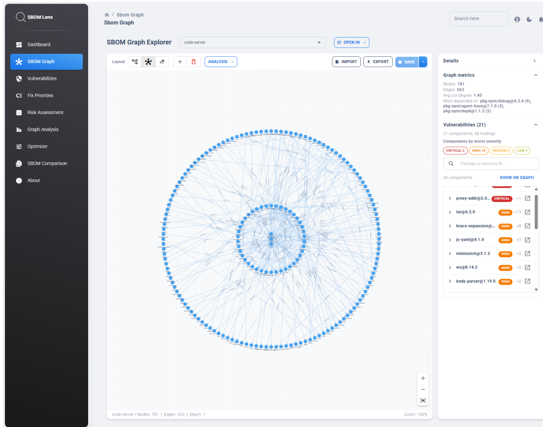
Figure 4.2: The SBOM Lens interface with the code-server SBOM loaded on the SBOM Graph page. The side navigation on the left links the pages of the application; the graph is drawn in the default radial layout, and the Details panel on the right summarises the graph and its vulnerabilities.
