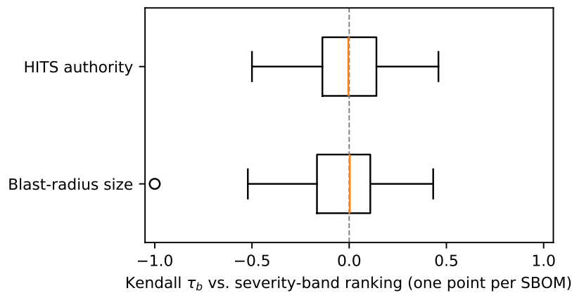
Figure 7.2: Kendall \tau_b between the severity-band ranking of each SBOM's vulnerable components and their ranking by blast-radius size (90 SBOMs) and by HITS authority (79 SBOMs).
