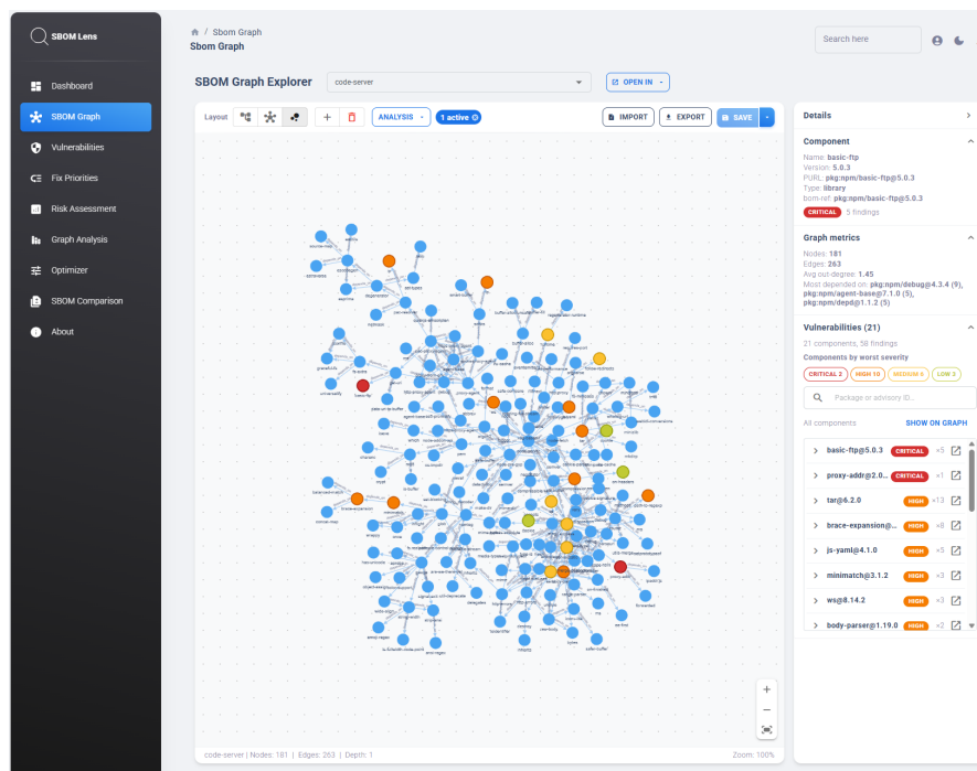
Figure 4.4: The code-server SBOM with the severity overlay of Section 5.5.1 active and basic-ftp selected. Vulnerable components are coloured by their worst severity band: red for CRITICAL, orange for HIGH, yellow for MEDIUM, and green-yellow for LOW. The Details panel shows the attributes of basic-ftp in the Component section, followed by the graph metrics and the vulnerable components of the SBOM.
