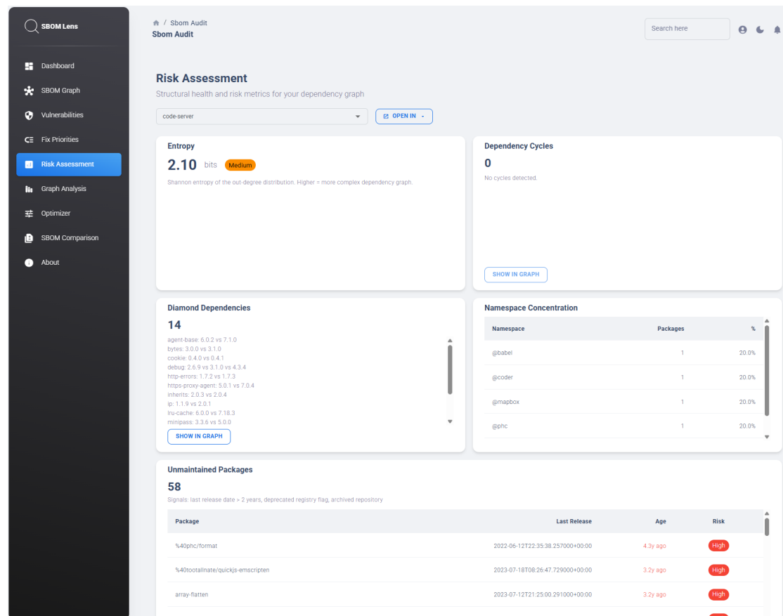
Figure 6.2: The Risk Assessment page for the code-server SBOM, showing the whole-graph audit: degree entropy, dependency cycles, version conflicts (labelled Diamond Dependencies in the interface), namespace concentration, and unmaintained packages.
