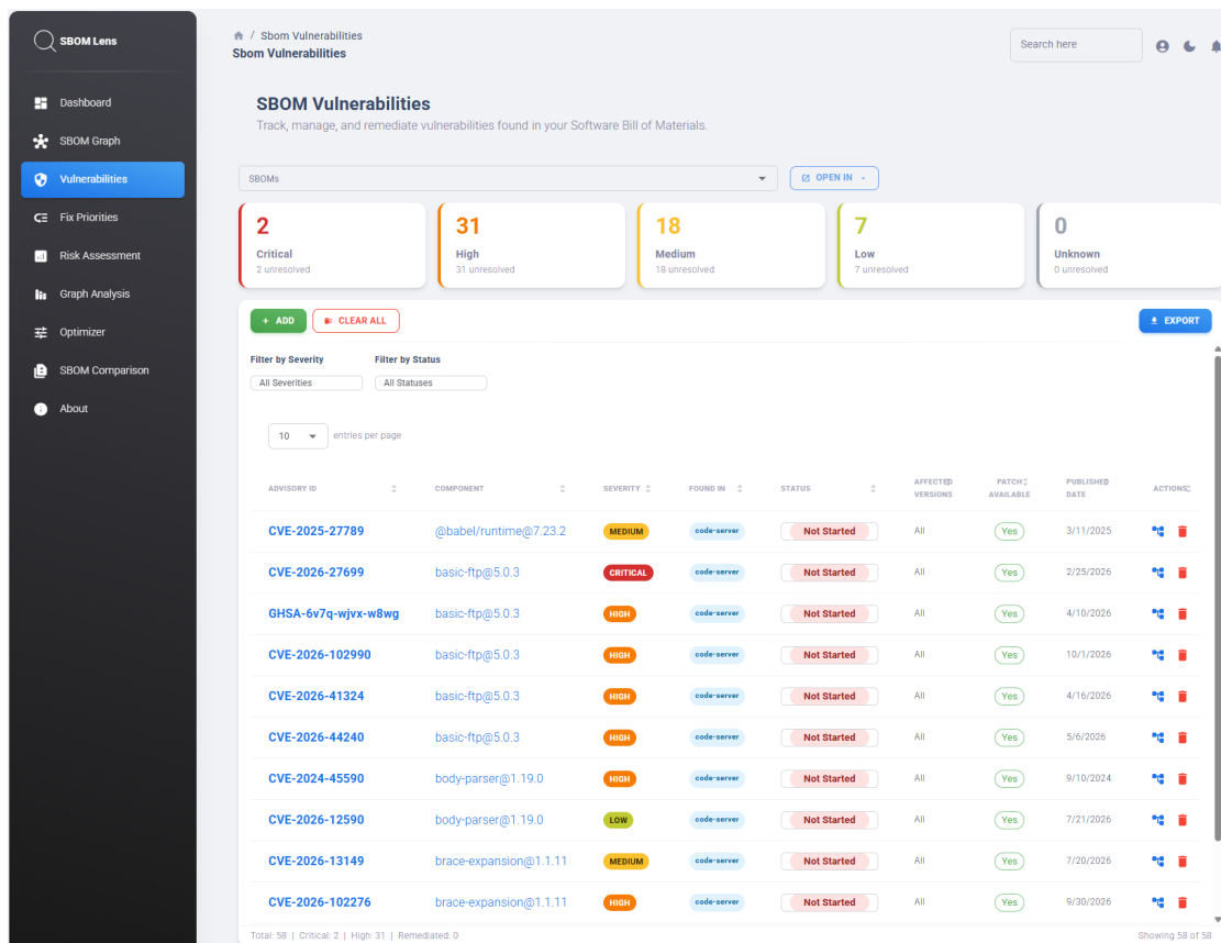
Figure 5.1: The Vulnerabilities page for the code-server SBOM: totals by severity band, and the stored vulnerability records with their component, severity band and remediation status.
