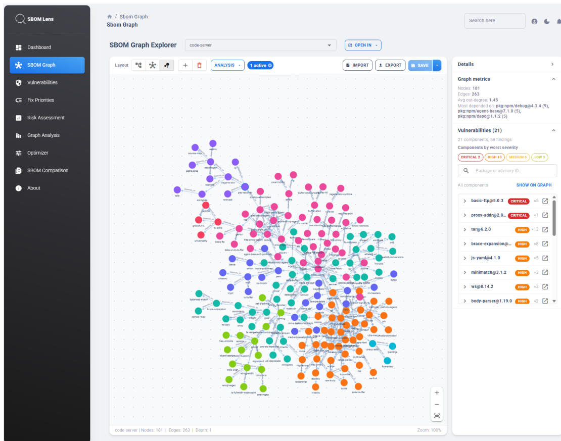
Figure 6.1: Louvain communities of the code-server dependency graph, one colour per community.
