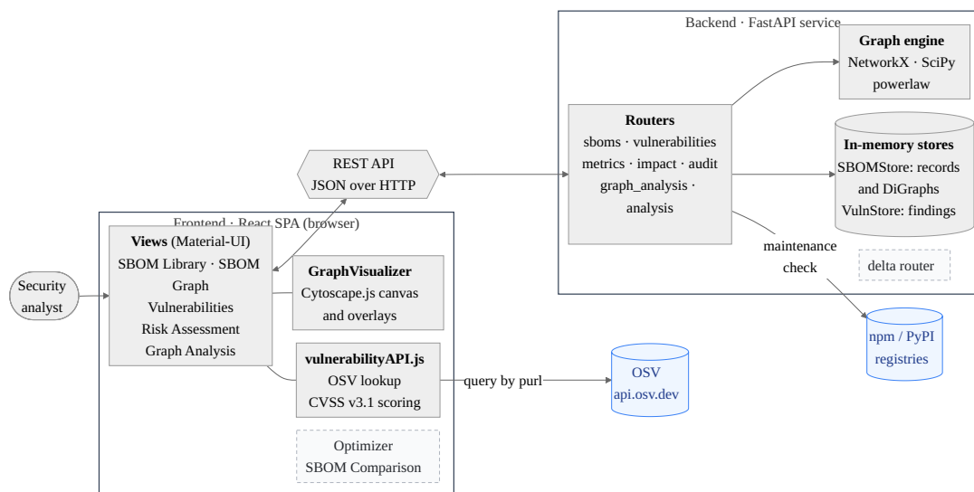
Figure 4.1: SBOM Lens three-layer architecture. Vulnerabilities are looked up in the browser and stored by the backend; the backend’s audit queries the package registries. Modules outside the thesis scope (Topology Optimiser, SBOM Comparison and the delta router) are drawn dashed.
