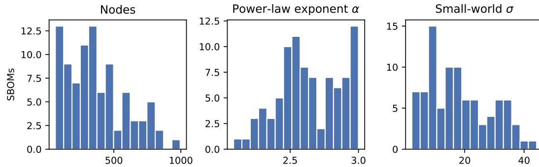
Figure 7.1: Distributions over the 90 SBOMs of the number of nodes, the fitted power-law exponent \alpha of the in-degree distribution (87 SBOMs), and the small-world coefficient \sigma .
