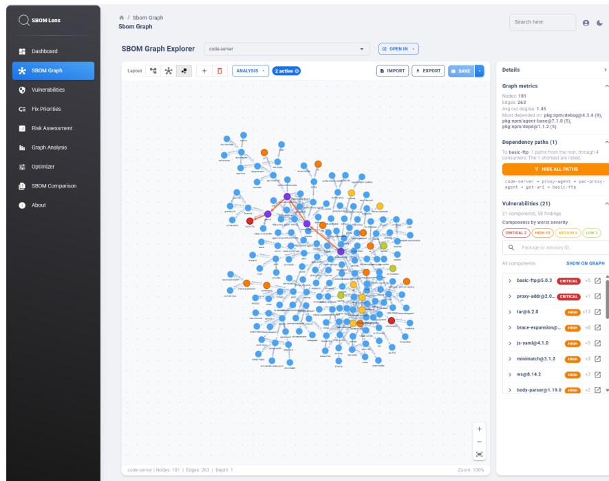
Figure 5.2: Blast radius of basic-ftp in the code-server SBOM. Its four consumers — get-uri , pac-proxy-agent , proxy-agent and the application code-server — are purple, basic-ftp keeps the red of its CRITICAL band, and the edges of the single dependency path are highlighted in orange. The Details panel lists the path, code-server → proxy-agent → pac-proxy-agent → get-uri → basic-ftp .
