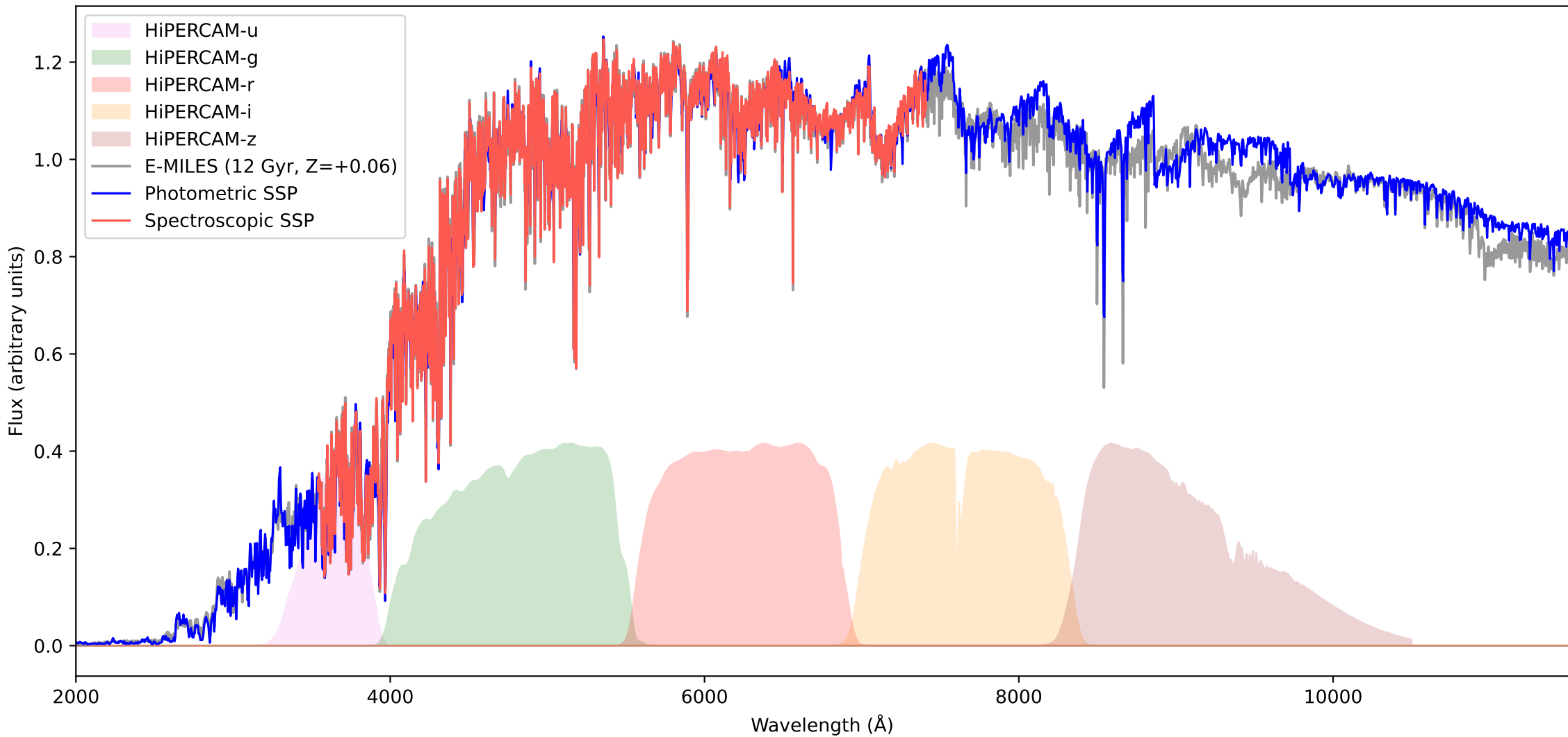
SSP Spectra with HiPERCAM Filter Responses
