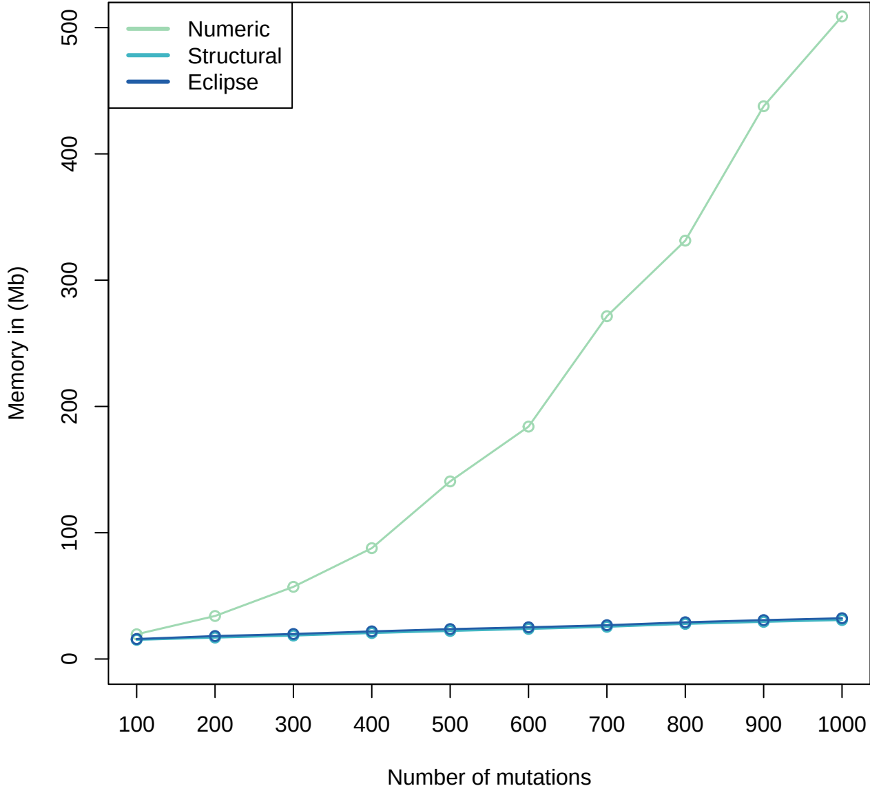
(A) Measuring memory consumption of different mutation counter
