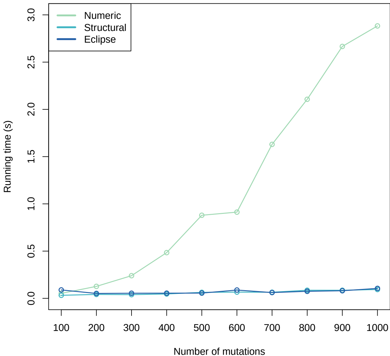
(A) Measuring execution time of different mutation counter
