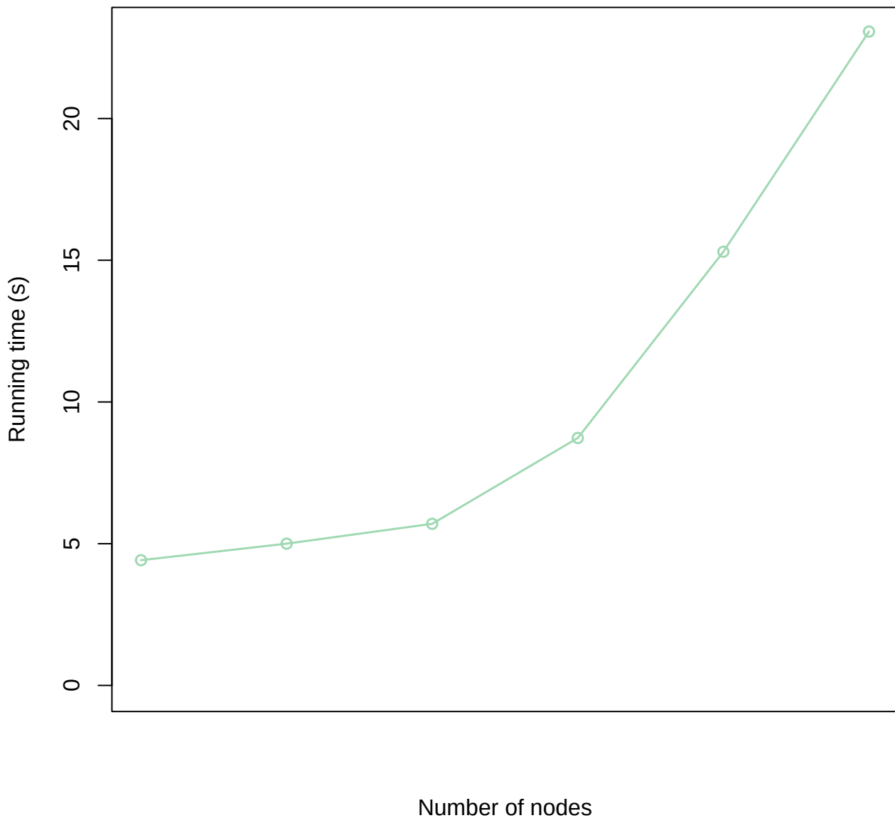
(A) Measuring execution time of Constant-Anaylsis example
