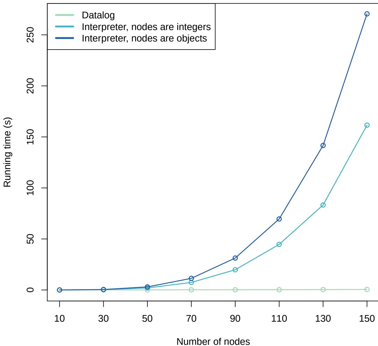
(A) Measuring execution time of right-recursive path example
