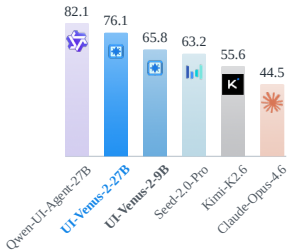
DeskCraft
