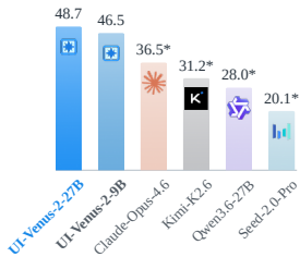
VenusBench-Mobile
