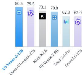
OSWorld-Verified
