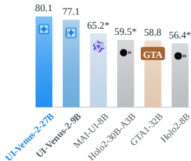
VenusBench-GD
