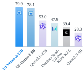
VenusBench-CAPTCHA
