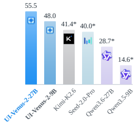
DeskCraft
