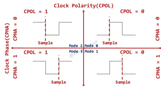
Figure 3: Timing diagram of sampling MISO and transmitting MOSI based on CPOL and CPHA
