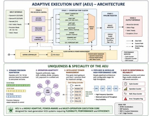
Figure 1: AEU architecture
