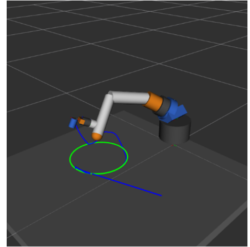
Fig. 6: Robot motion without manipulability optimization - tracking failure due to singularities
