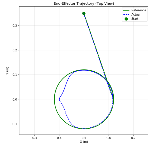
Fig. 2: Top view of circular cleaning trajectory in XY plane
