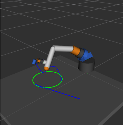
Fig. 6: Robot motion without manipulability optimization - tracking failure due to singularities
