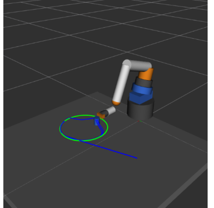
Fig. 5: Robot motion with manipulability optimization - stable tracking
