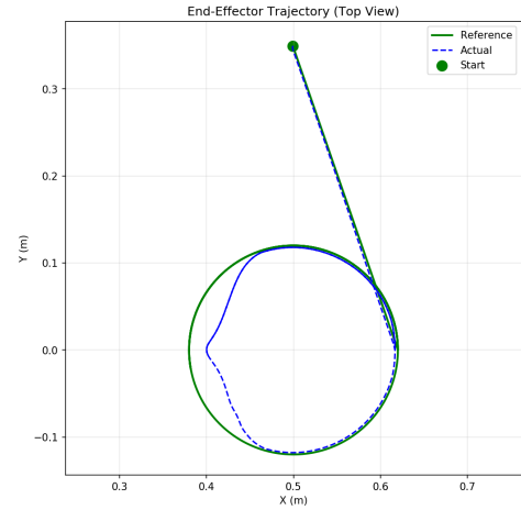
Fig. 1: Top view of circular cleaning trajectory in XY plane
