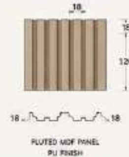
5. FLUTED PANEL DETAIL
