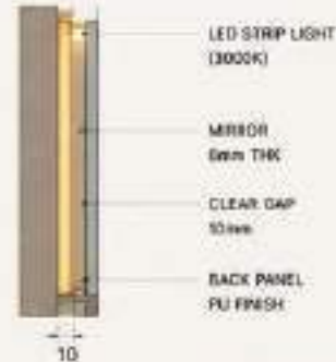
6. MIRROR & LED DETAIL (SECTION)
