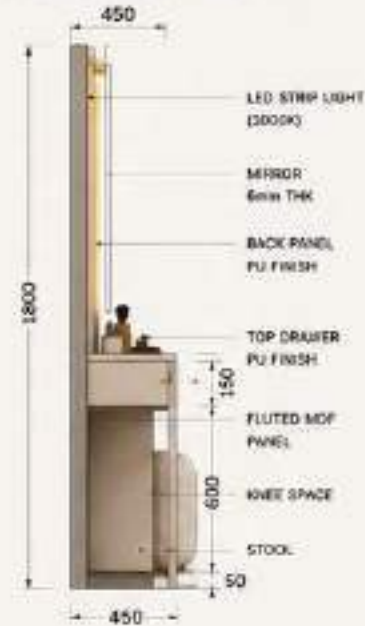
2. SIDE ELEVATION (SECTION)
