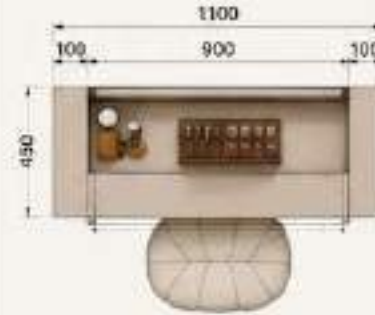
3. PLAN VIEW (TOP)
