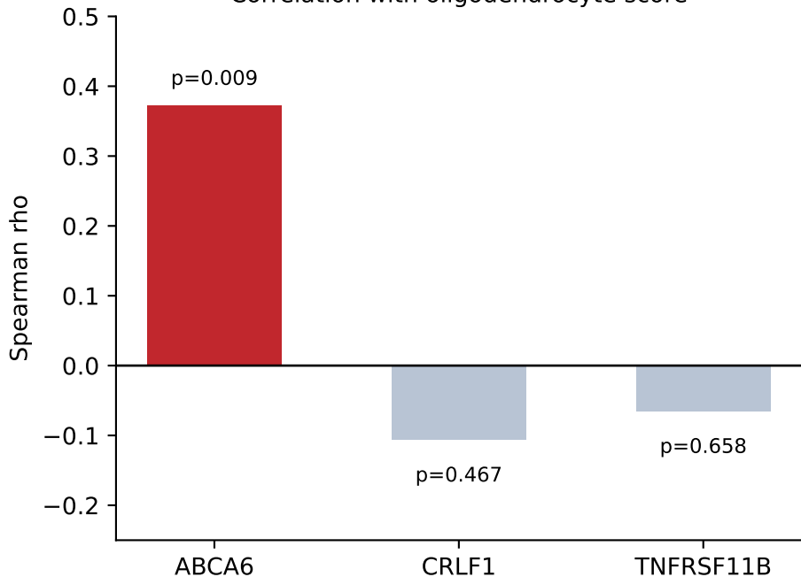
Correlation with oligodendrocyte score
