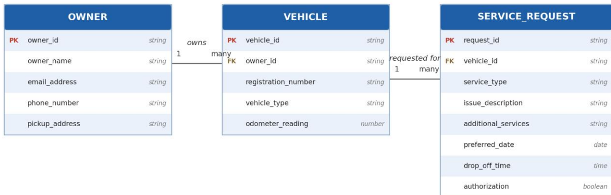
ER Diagram — Vehicle Service Request System
