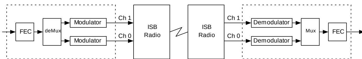
FIGURE F-4. 2-ISB Modem.
