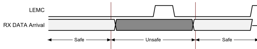
Figure 28: LEMC Margin
