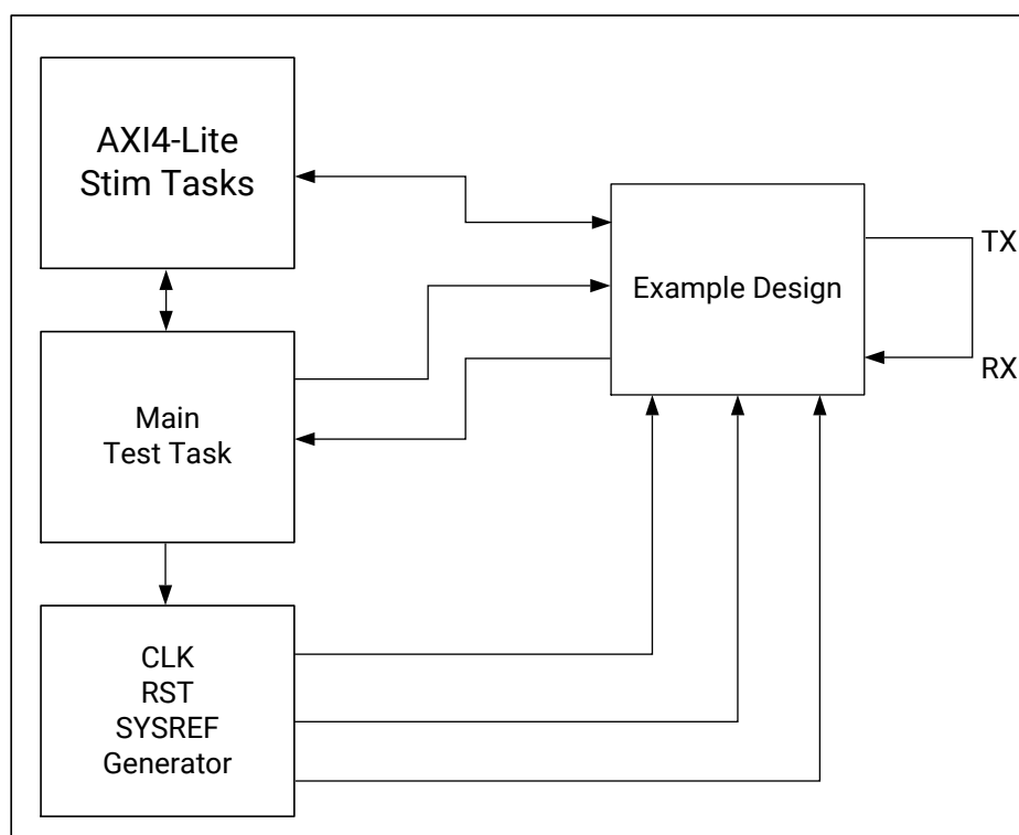
Figure 53: Core Demo Test Bench
