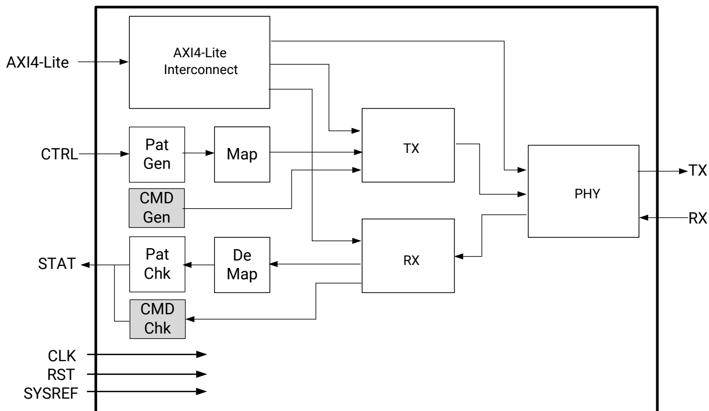
Figure 52: Core Example Design for UltraScale+/UltraScale Devices
