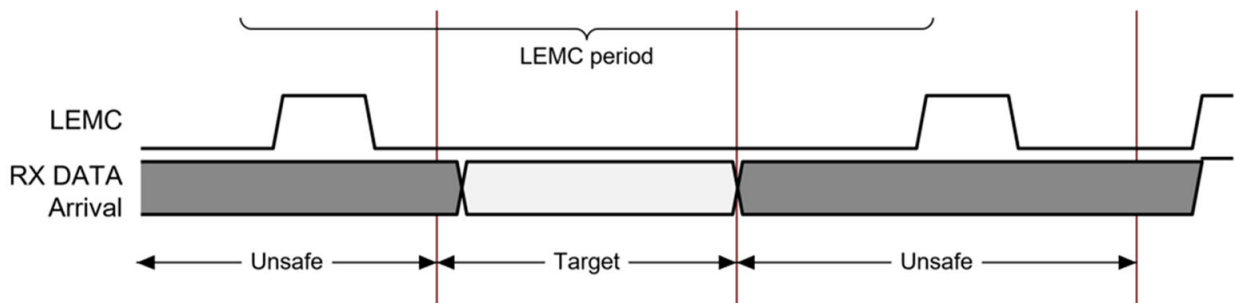
Figure 29: Target Window
