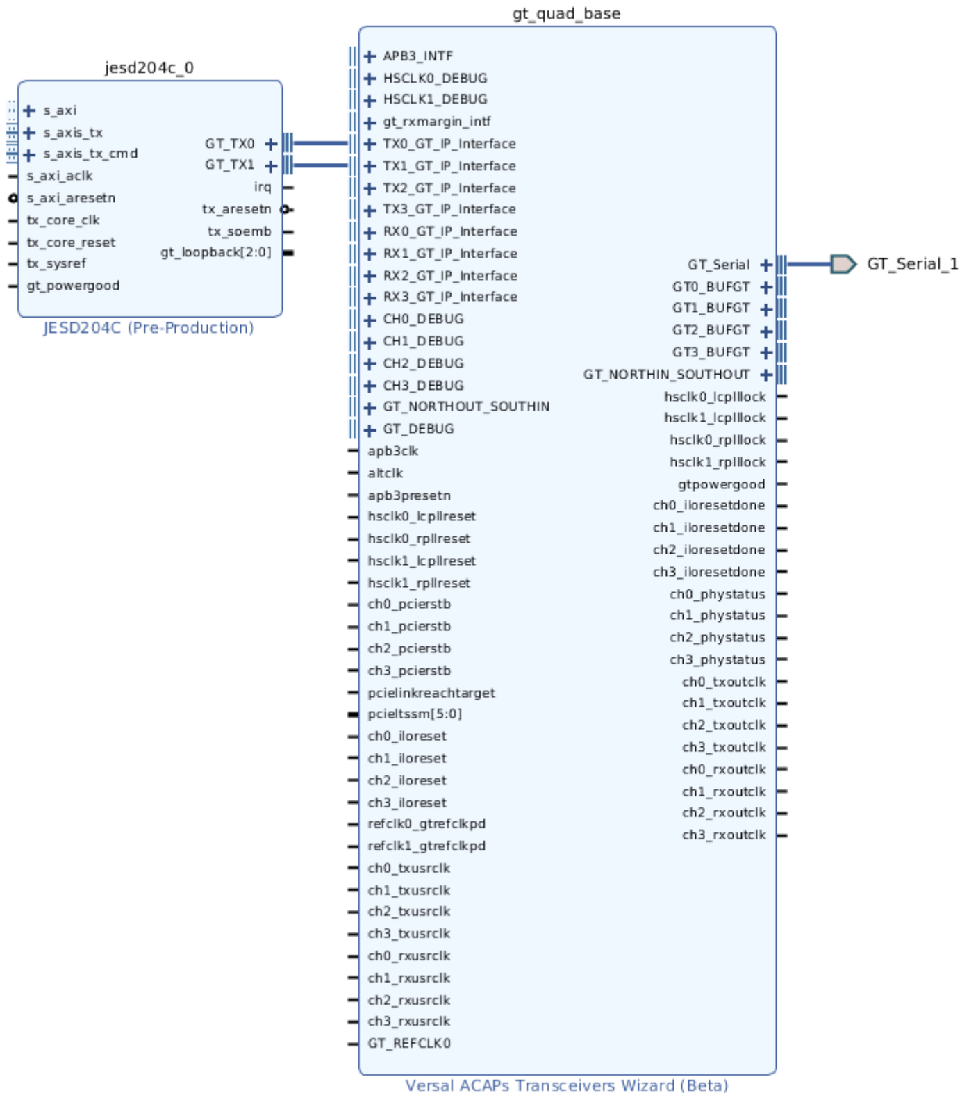
Figure 45: Block Automation on a Single JESD204C Core with Default Settings
