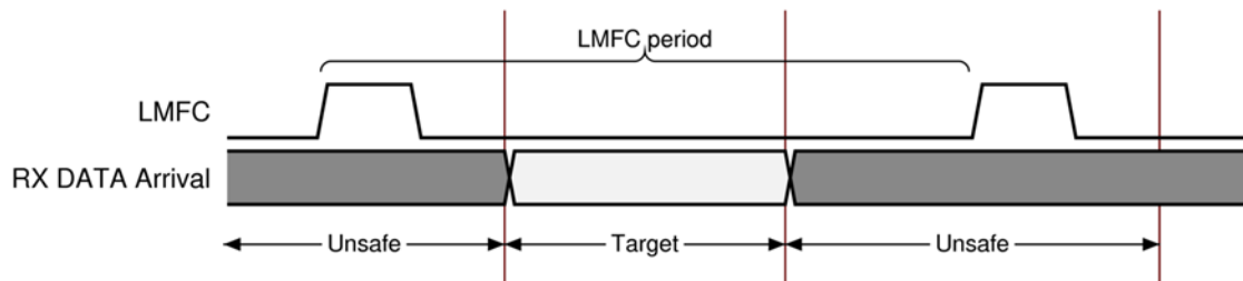
Figure 26: Target Window
