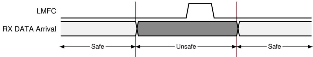
Figure 25: LMFC Margin
