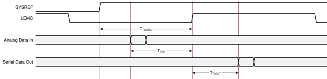
Figure 21: ADC Timing
