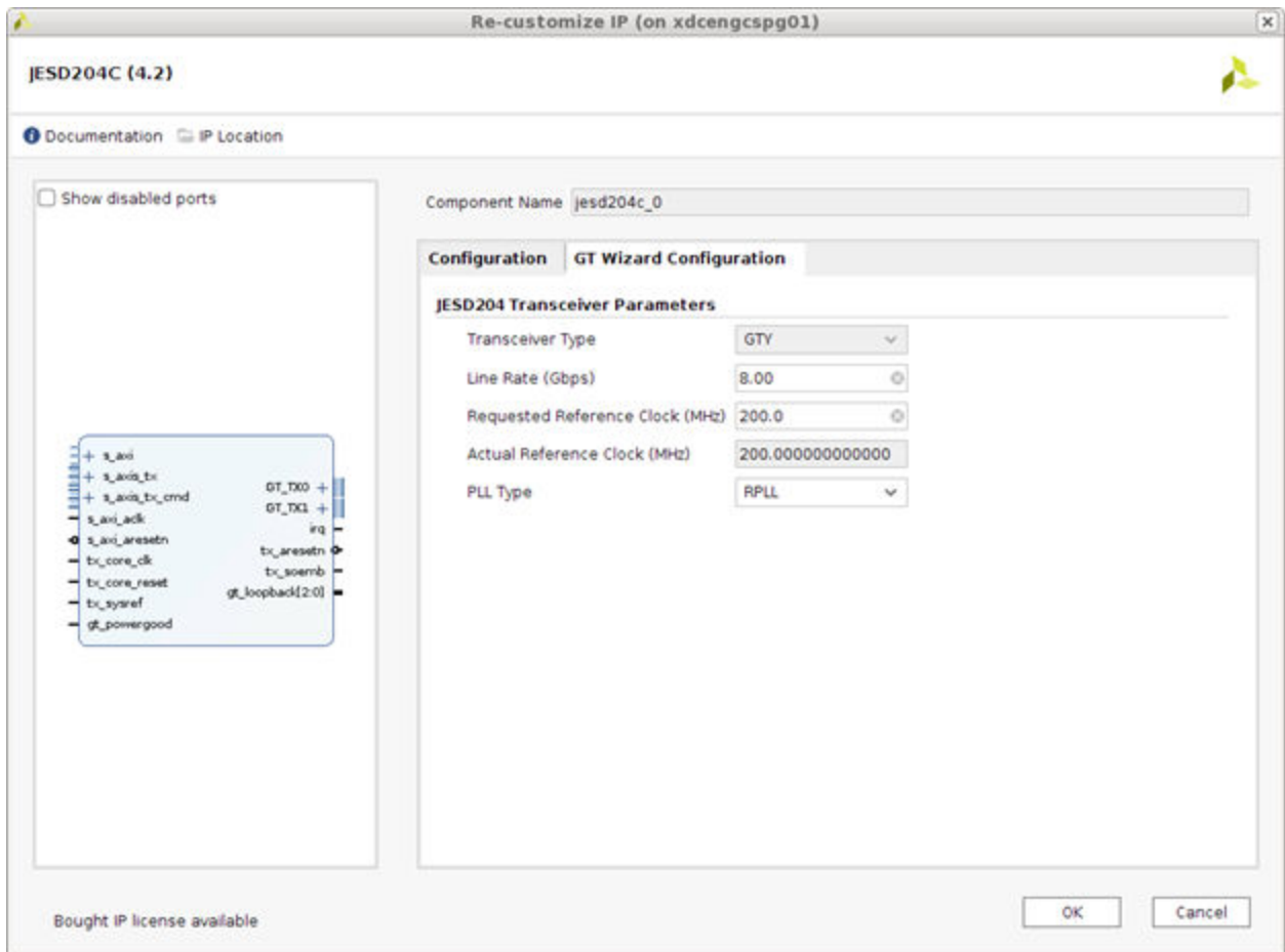
Figure 40: GT Wizard Configuration Tab
