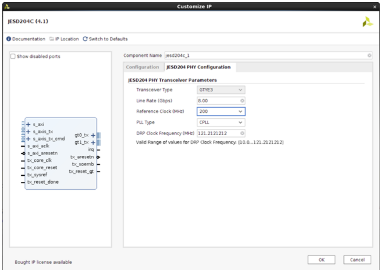
Figure 41: JESD204 PHY Tab
