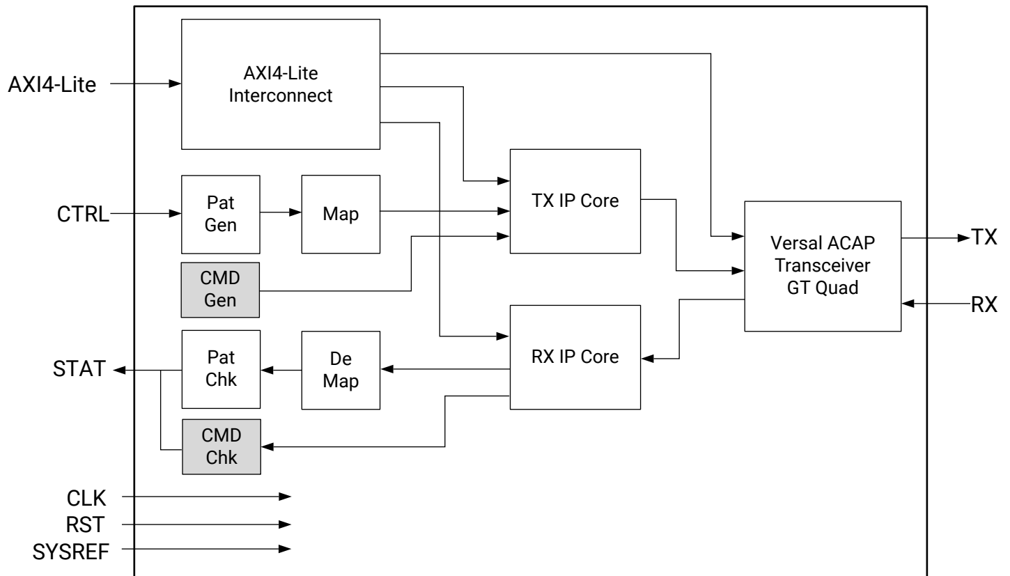
Figure 51: Core Example Design for Versal ACAPs
