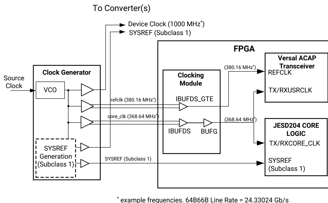
Figure 1: Separate Transceiver Reference and Core Clocks: 64B66B Example for Versal ACAPs
