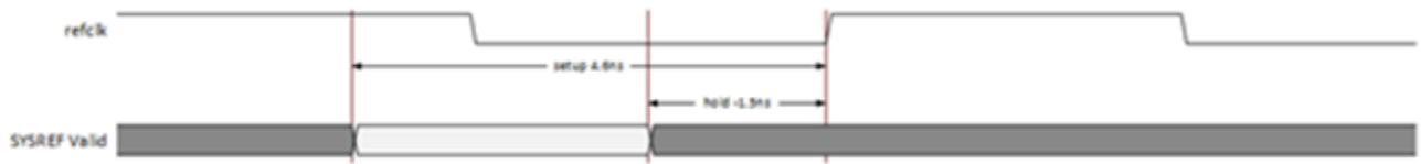
Figure 17: SYSREF Timing Example
