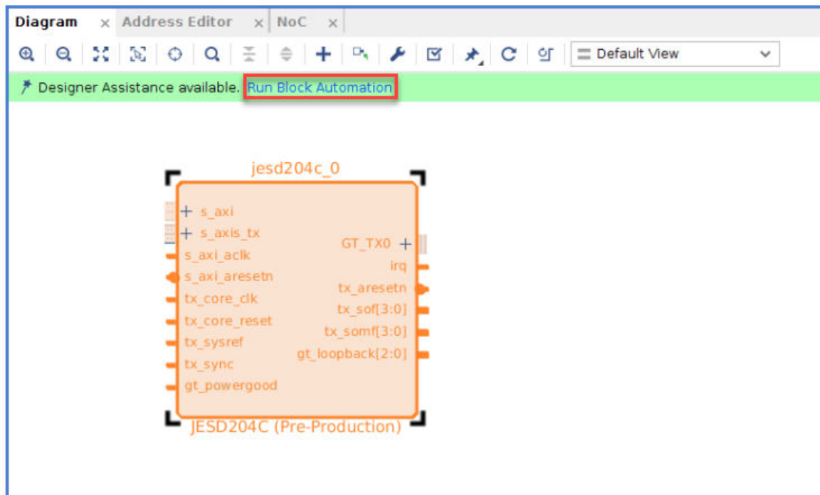
Figure 43: Block Automation Link for Versal ACAPs
