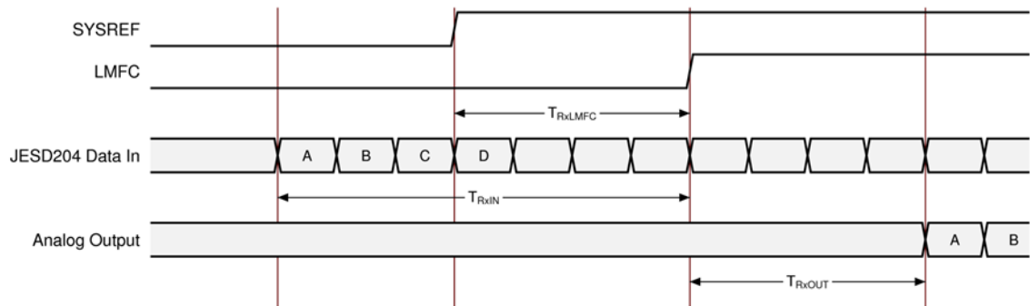
Figure 33: DAC RX Timing
