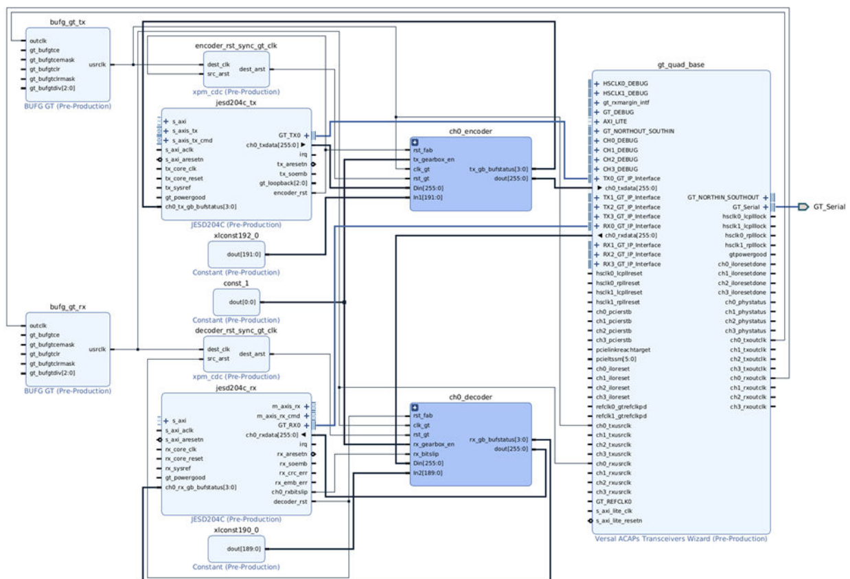
Figure 47: Block Automation on TX and RX JESD204C Cores on Versal ACAP GTM Transceivers
