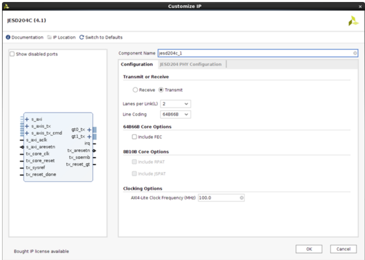
Figure 39: Configuration Tab for UltraScale+/UltraScale Devices
