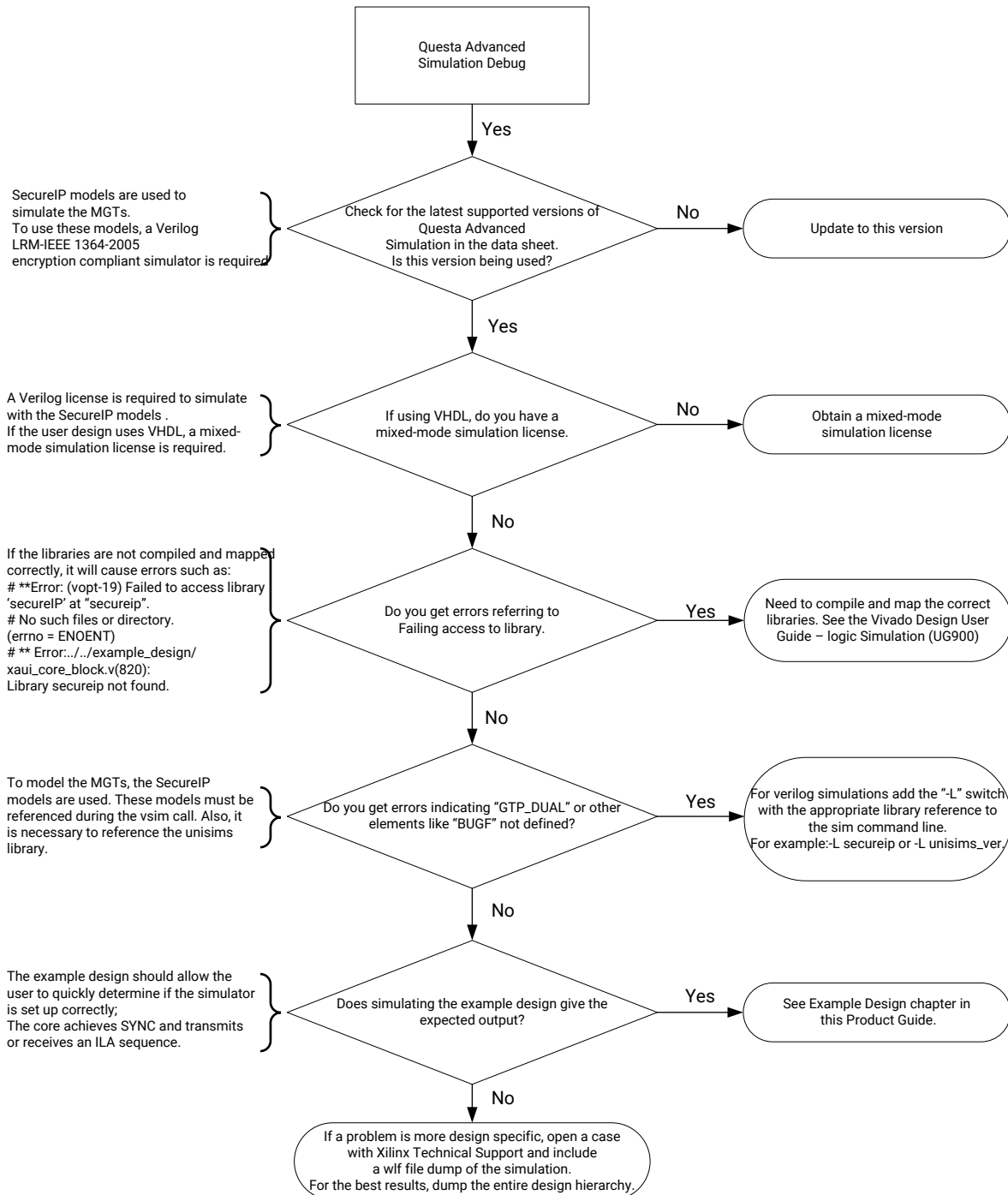
Figure 54: Simulator Flow Diagram
