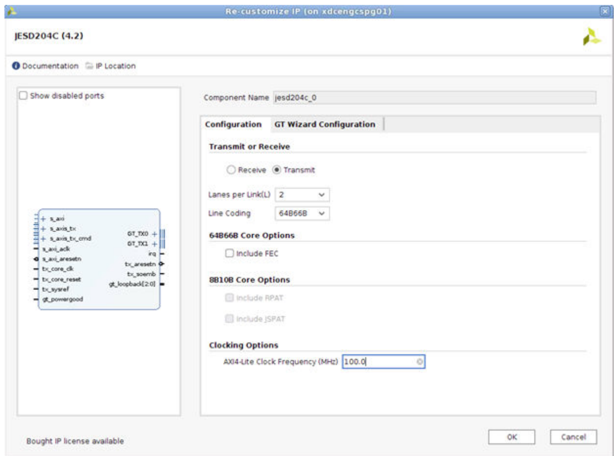
Figure 38: Configuration Tab for Versal ACAPs
