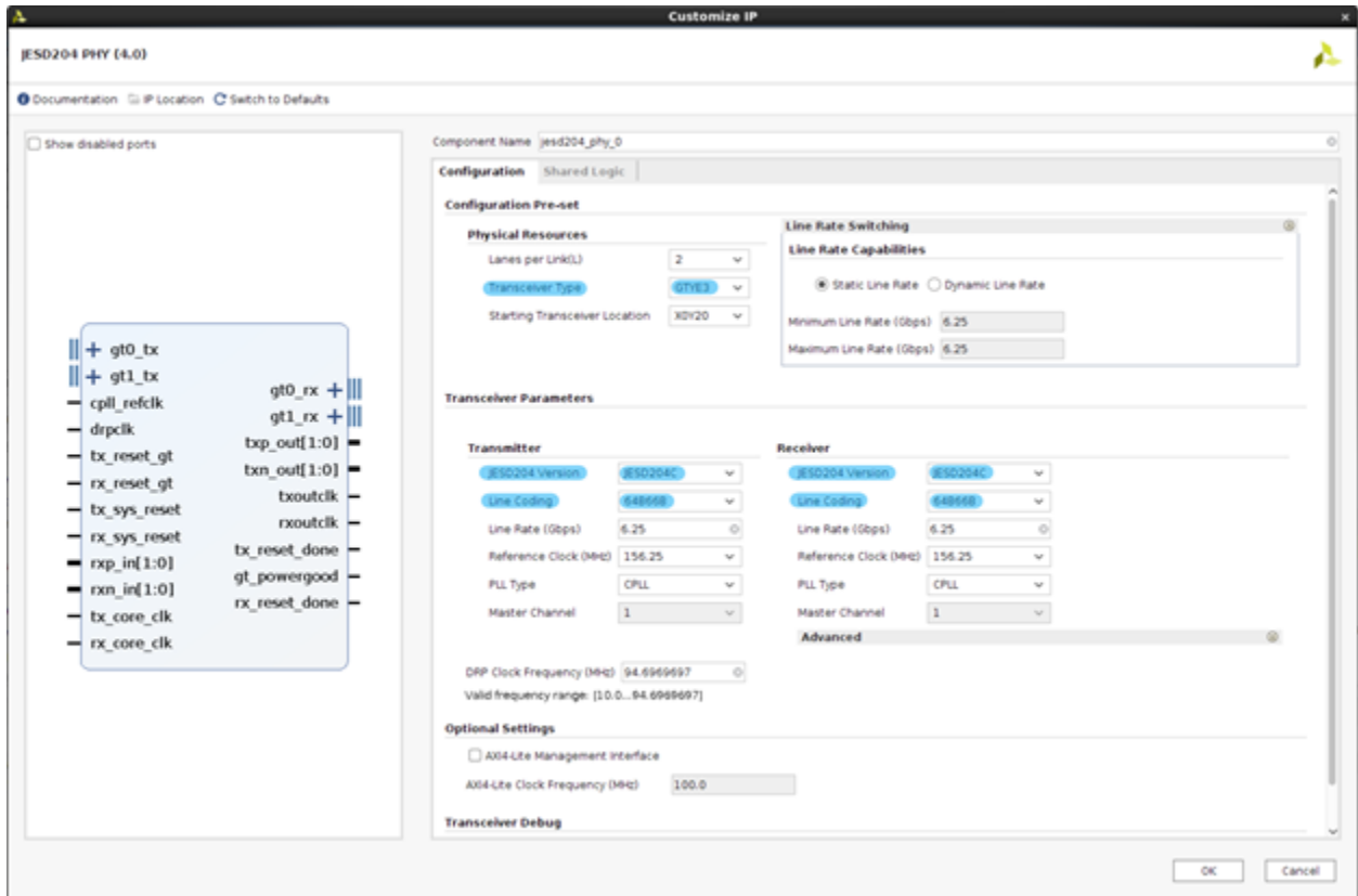
Figure 48: JESD204 PHY GUI
