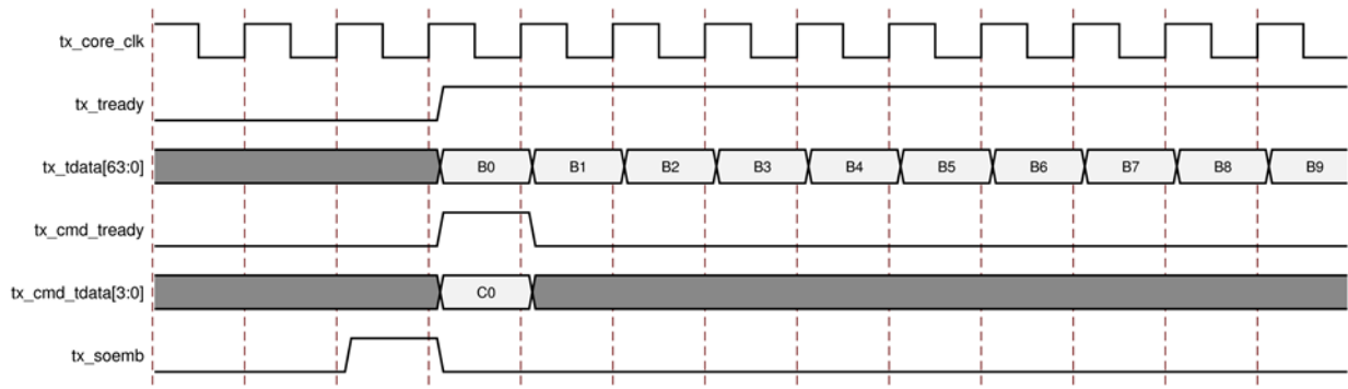
Figure 13: 64B66B Transmit Data Interface Timing
