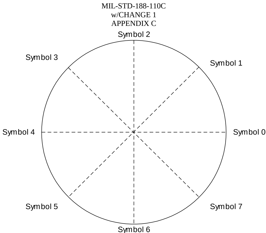
FIGURE C- 1. 8PSK signal constellation and symbol mapping.
