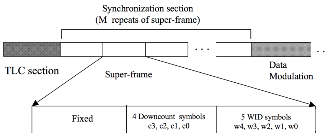
FIGURE D-8. Synchronization preamble structure.
