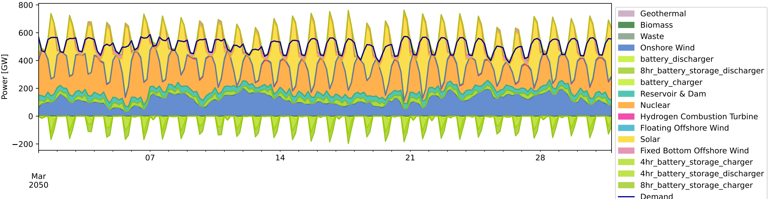
Production [GW] (interconnect = usa | #clusters = 134 | ll = v1.0 | opts = 4H | sectors = E)
