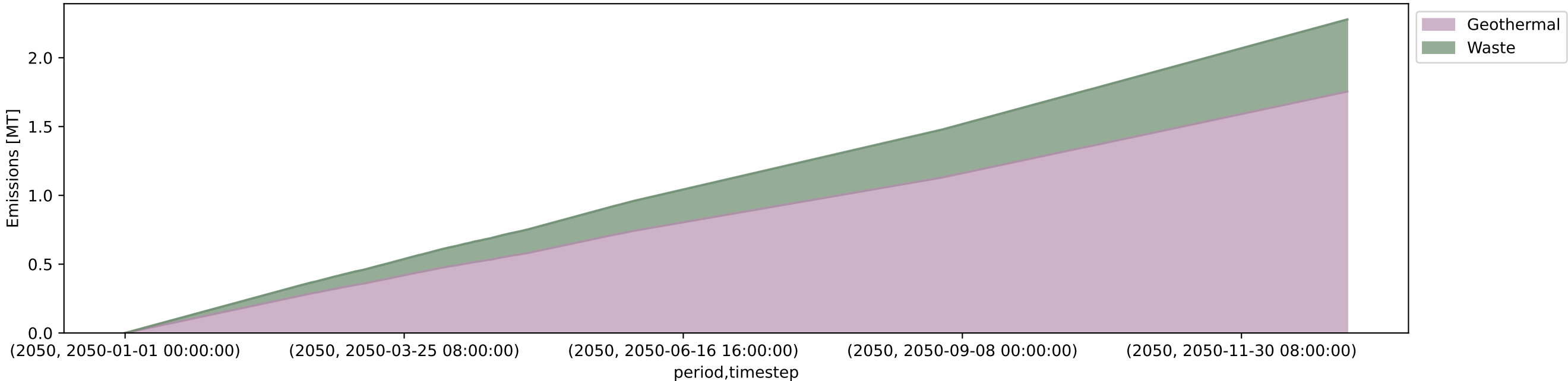
Technology Accumulated Emissions (interconnect = usa | #clusters = 134 | ll = v1.0 | opts = 1H | sectors = E)
