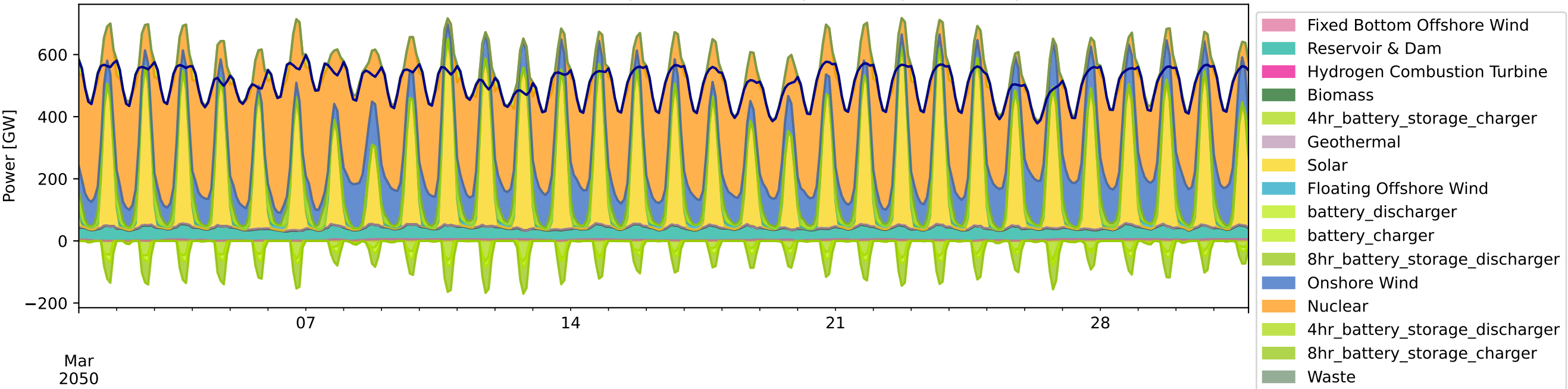
Production [GW] (interconnect = usa | #clusters = 134 | ll = v1.0 | opts = 2H | sectors = E)
