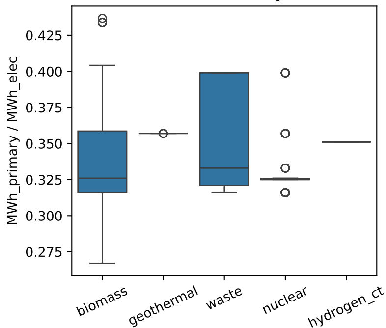
Plant Efficiency
