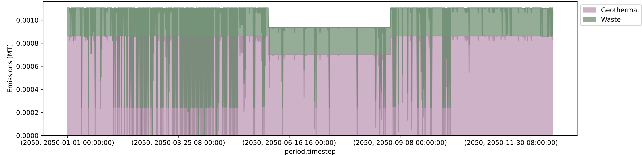
Technology Emissions (interconnect = usa | #clusters = 134 | ll = v1.0 | opts = 4H | sectors = E)
