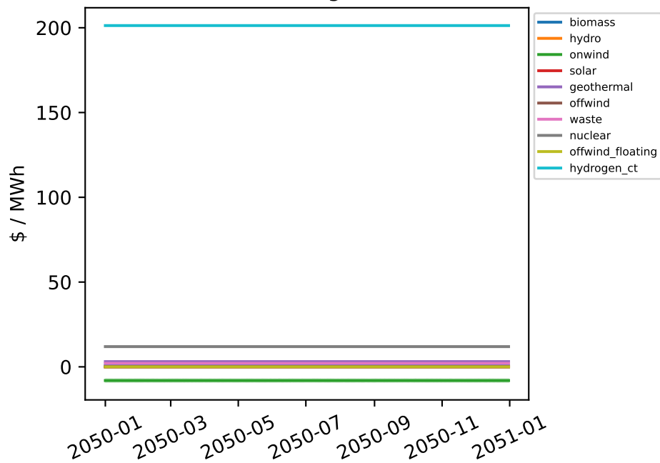
Generator Marginal Costs
