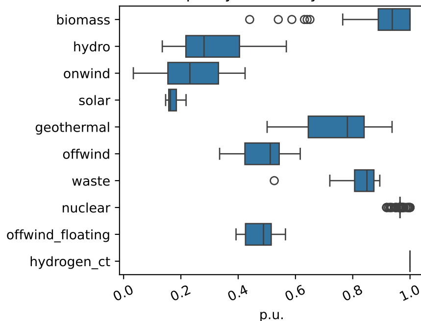
Capacity Factors by Carrier
