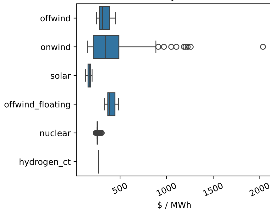
LCOE by Carrier
