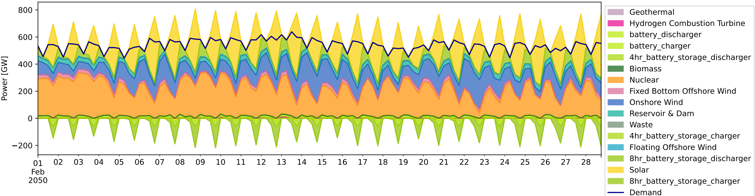
Production [GW] (interconnect = usa | #clusters = 134 | ll = v1.0 | opts = 6H | sectors = E)
