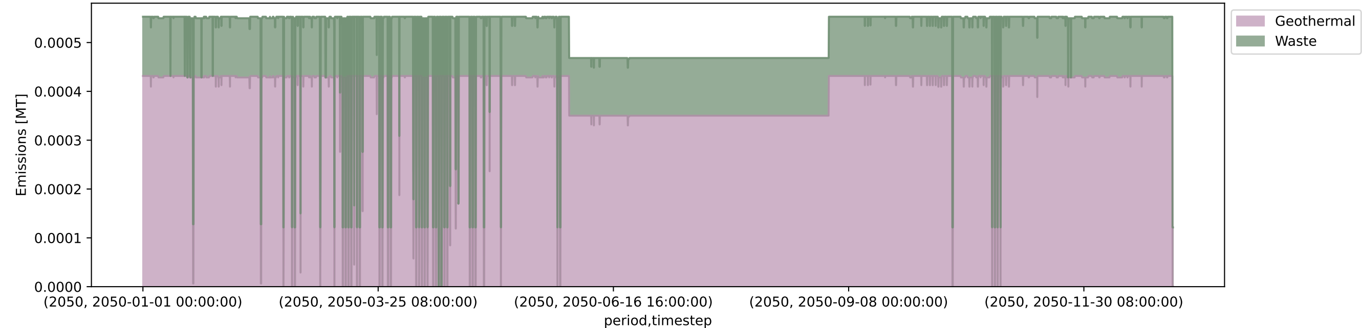
Technology Emissions (interconnect = usa | #clusters = 134 | ll = v1.0 | opts = 2H | sectors = E)
