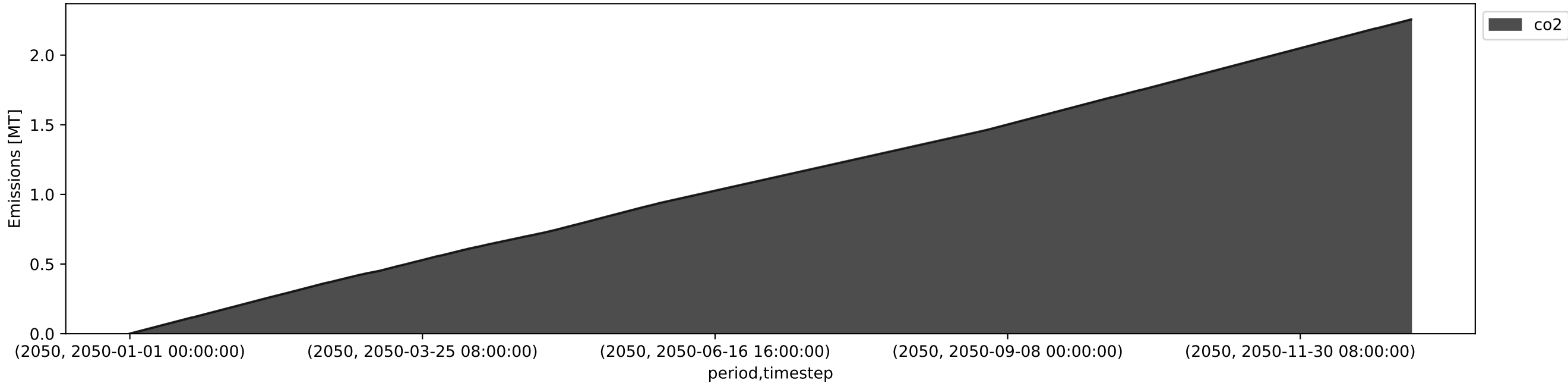
Accumulated Emissions (interconnect = usa | #clusters = 134 | ll = v1.0 | opts = 2H | sectors = E)
