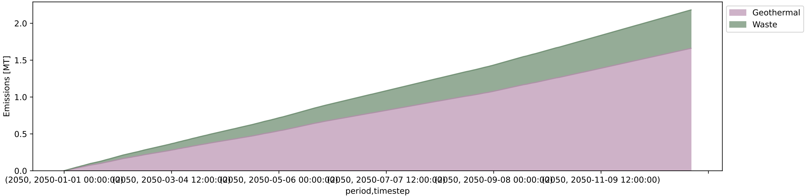
Technology Accumulated Emissions (interconnect = usa | #clusters = 134 | ll = v1.0 | opts = 3H | sectors = E)
