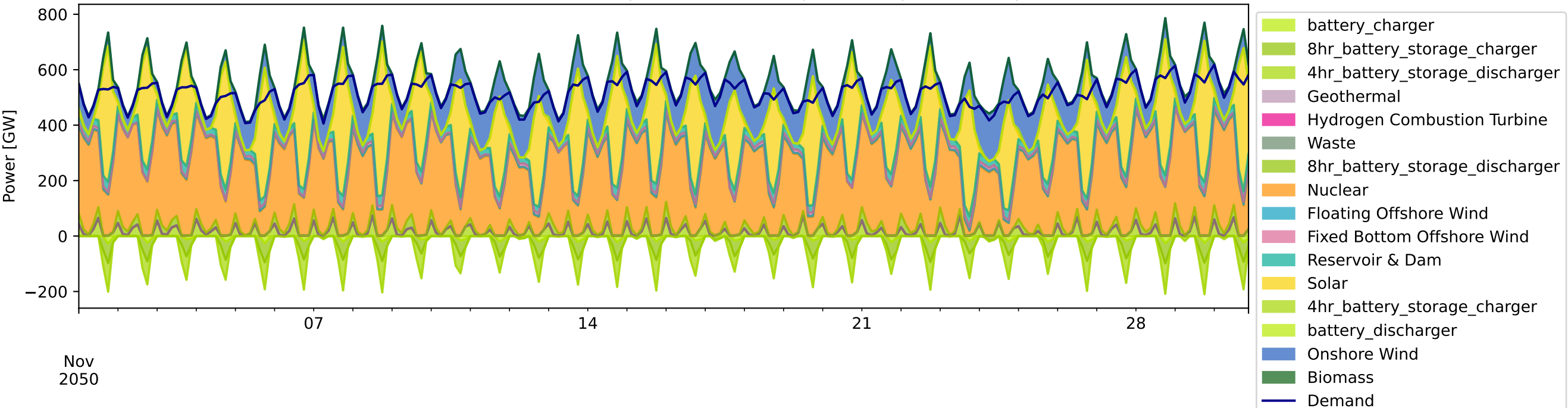
Production [GW] (interconnect = usa | #clusters = 134 | ll = v1.0 | opts = 3H | sectors = E)
