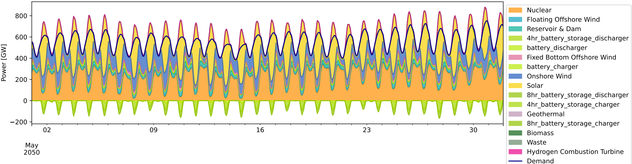
Production [GW] (interconnect = usa | #clusters = 134 | ll = v1.0 | opts = 1H | sectors = E)
