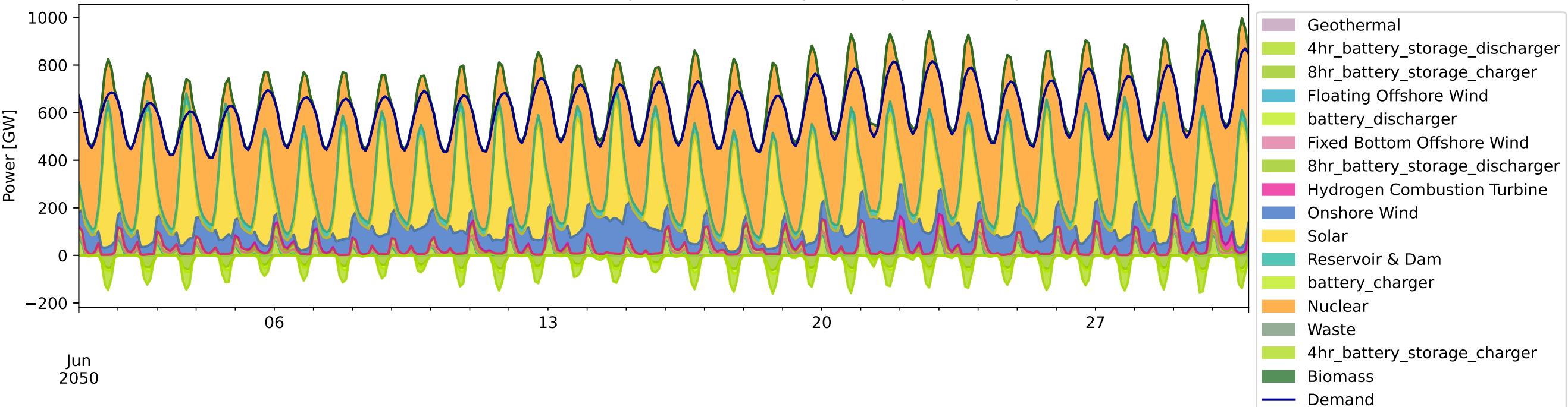
Production [GW] (interconnect = usa | #clusters = 134 | ll = v1.0 | opts = 2H | sectors = E)
