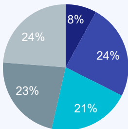
Grade Distribution
