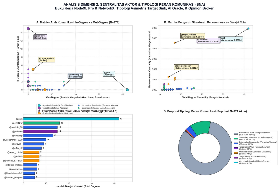
Figure 3: Four-Quadrant Actor Centrality Typology
