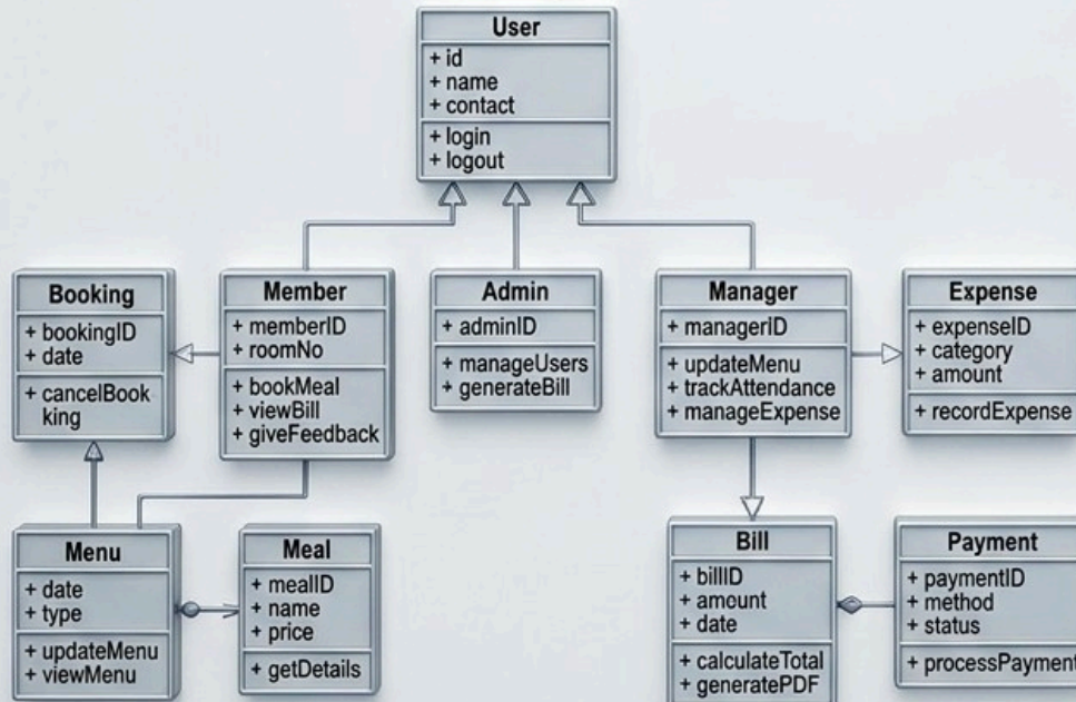
Class Diagram
