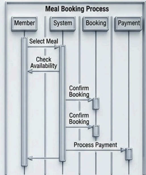
Sequence Diagrams
