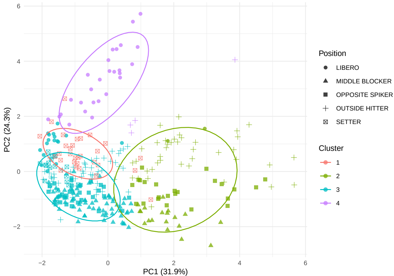
K-means solution (k = 4)
