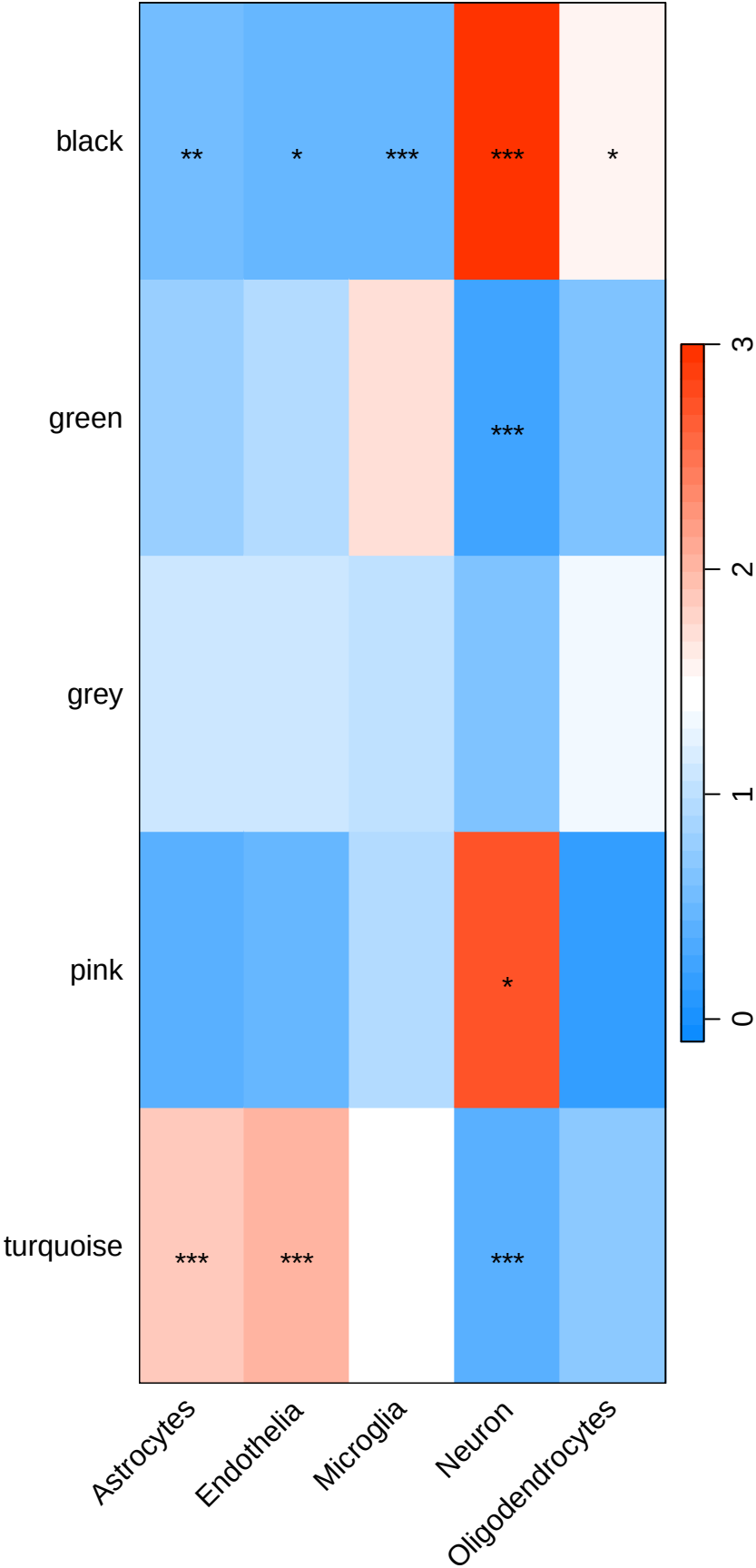
Cell-type enrichment Heatmap
