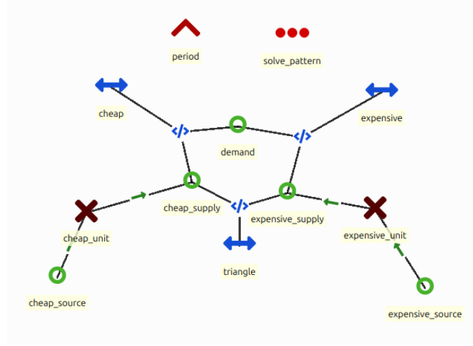
Figure 10: Implementation of unit commitment in the ines-spec.
