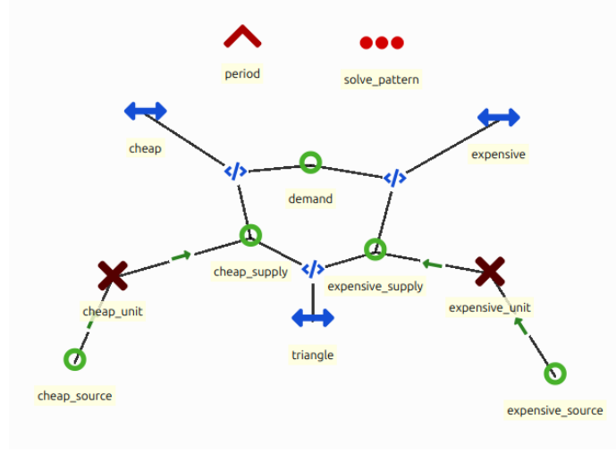
Figure 8: Implementation of investment = fixed in the ines-spec.
