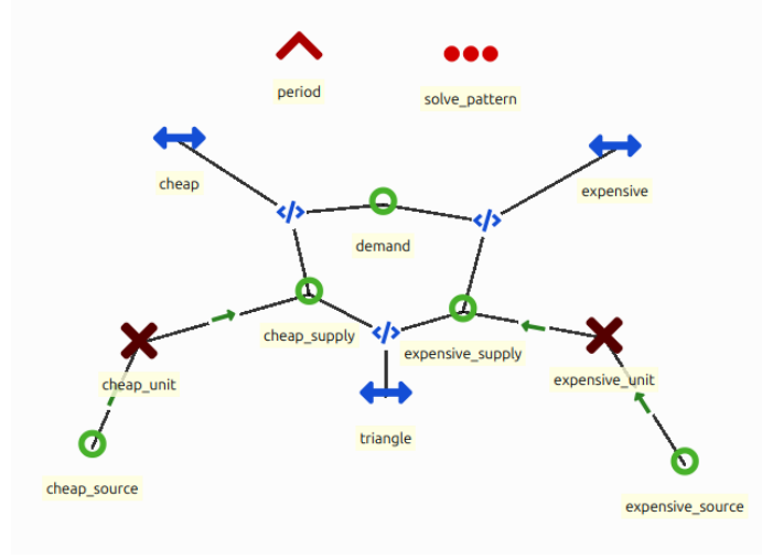
Figure 2: Implementation of network = mesh in the ines-spec.
