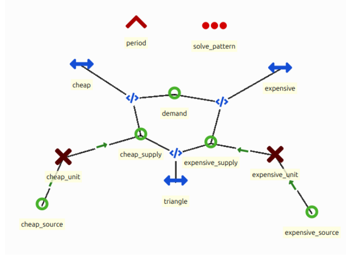
Figure 3: Implementation of resolution = fixed in the ines-spec.
