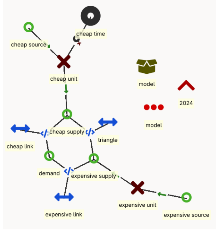
Figure 2.4: Implementation of resolution = flexible in the ines spec.
