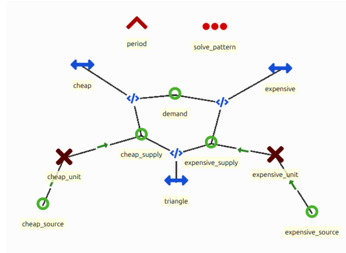
Figure 2.9: Implementation of unit commitment in the ines spec.
