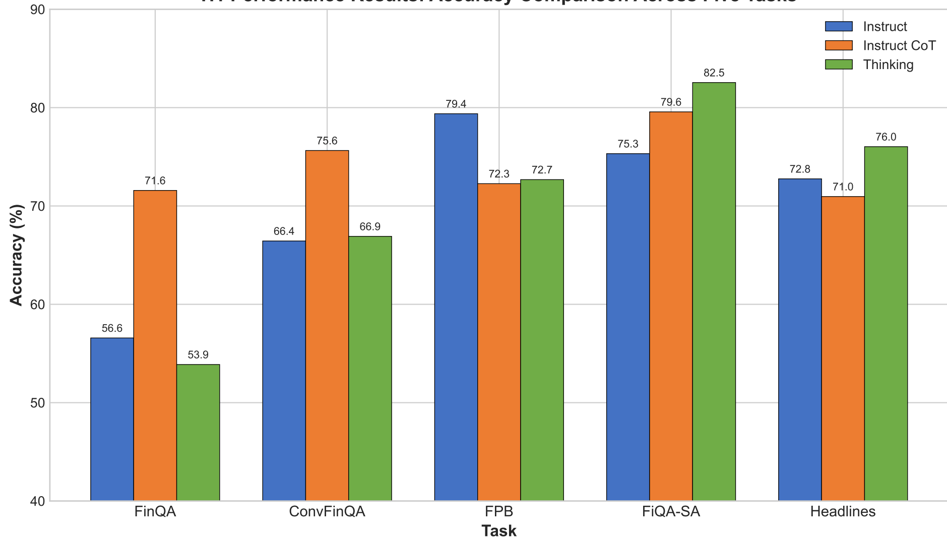
H1 Performance Results: Accuracy Comparison Across Five Tasks
