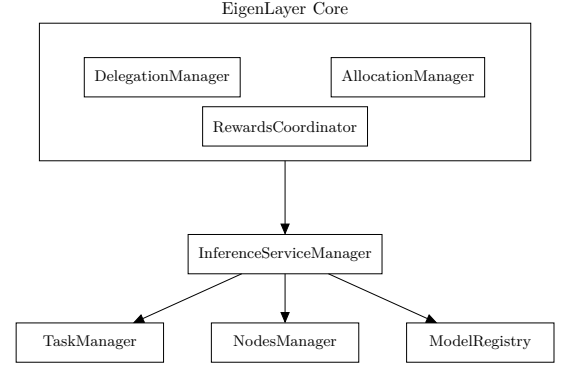
Fig. 3. EigenLayer Integration Architecture
