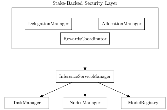
Fig. 3. Security Integration Architecture
