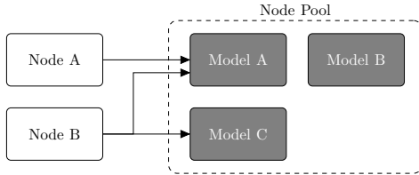
Fig. 4. Model Registration
