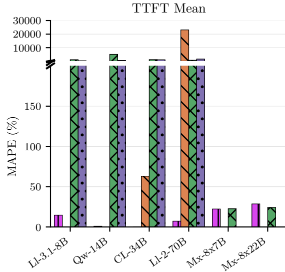
Prediction Error Across Model Architectures (All Simulators) ↓
