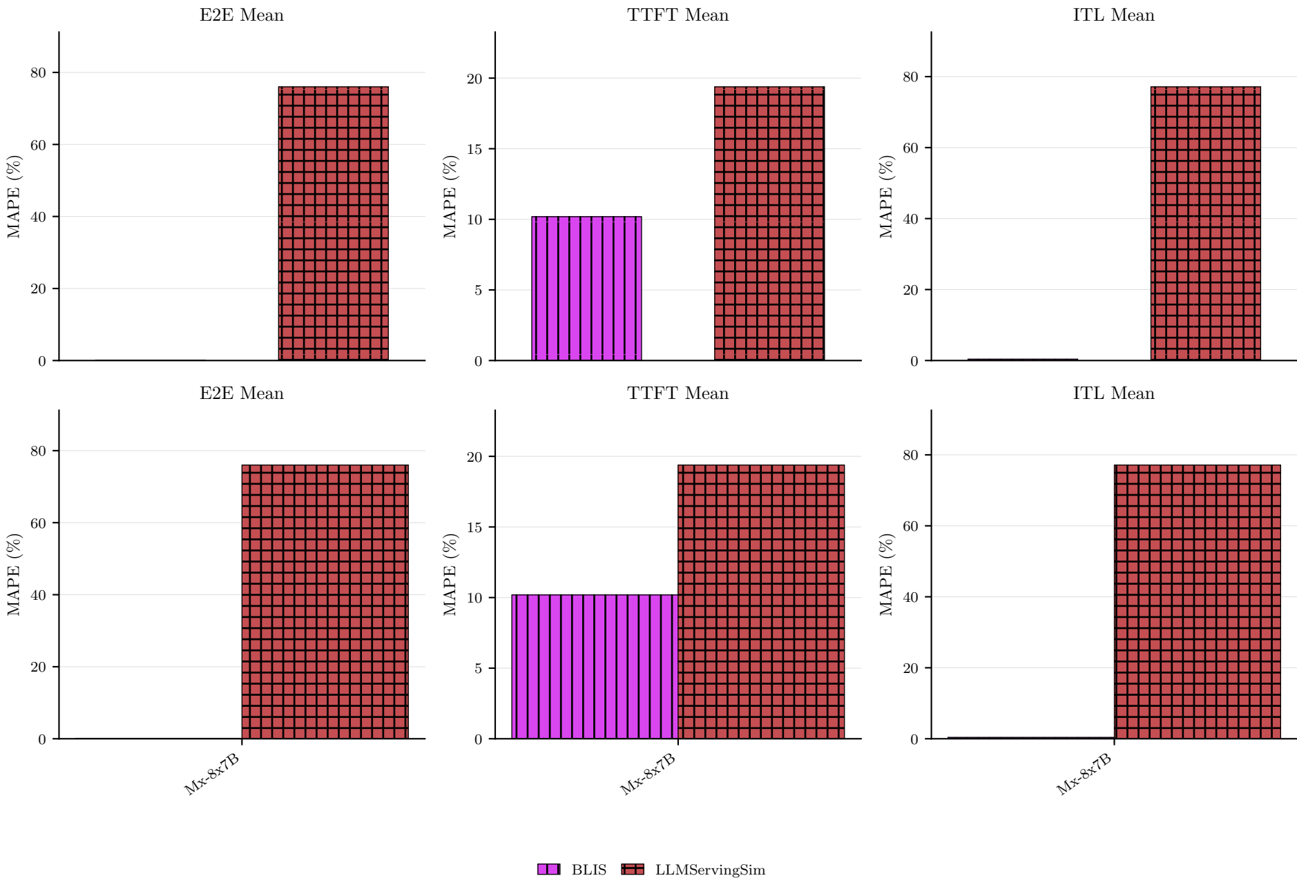
BLIS vs LLMservingSim Simulator Comparison (n=1) ↓
