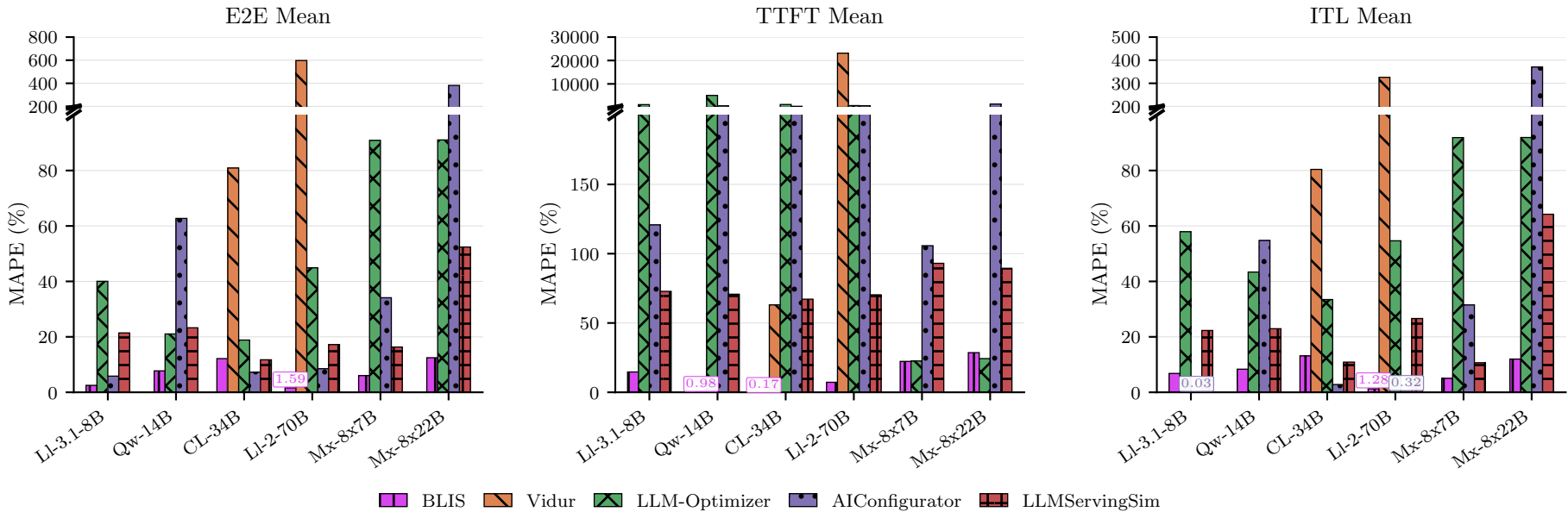
Prediction Error Across Model Architectures (All Simulators) ↓
