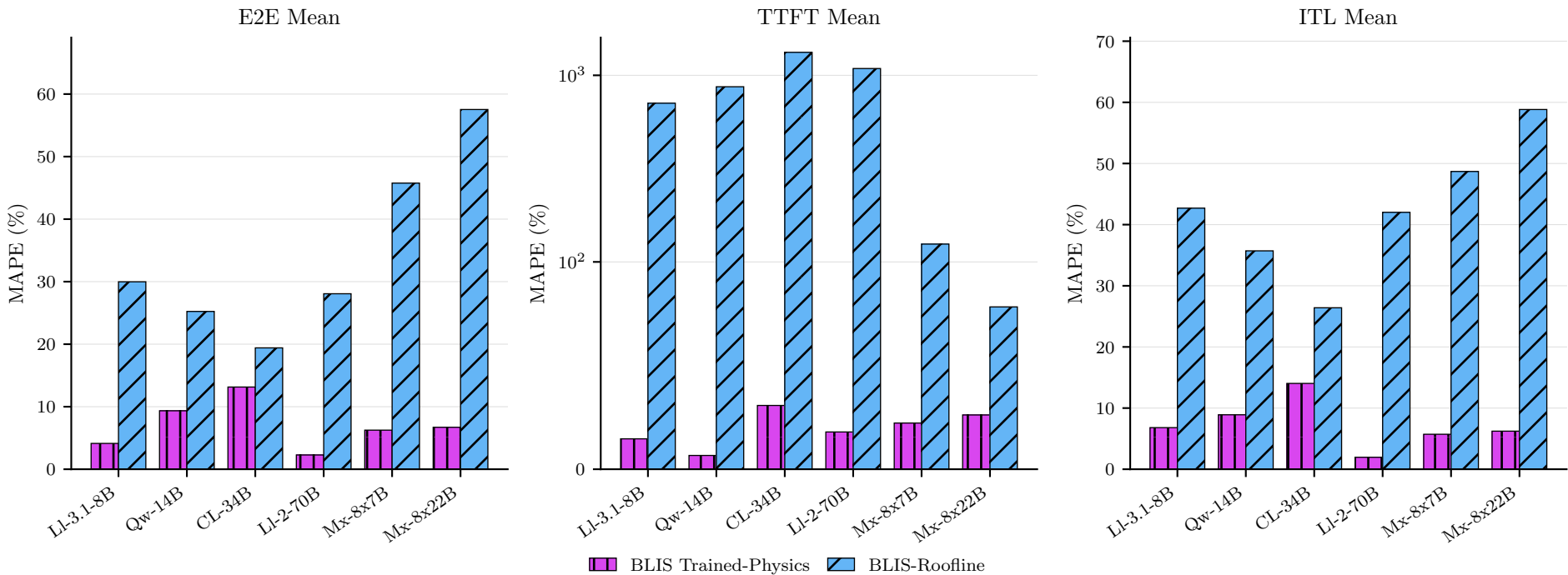
BLIS-Roofline vs BLIS Trained-Physics Simulator Comparison (n=38) ↓
