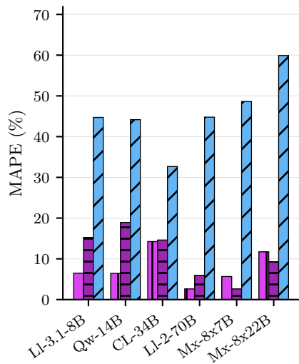
ITL Mean
