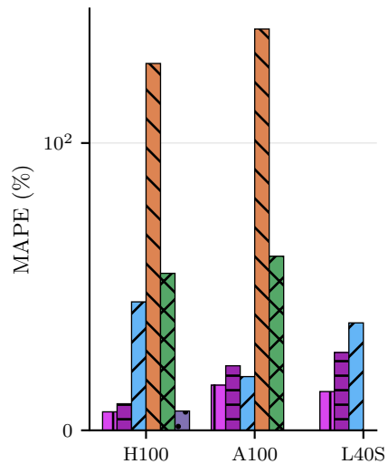
ITL Mean
