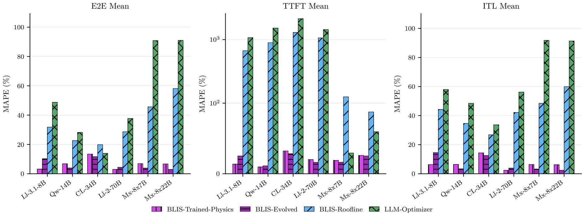
BLIS-Roofline &amp; BLIS-Trained-Physics &amp; BLIS-Evolved vs LLM-Optimizer (n=36) ↓
