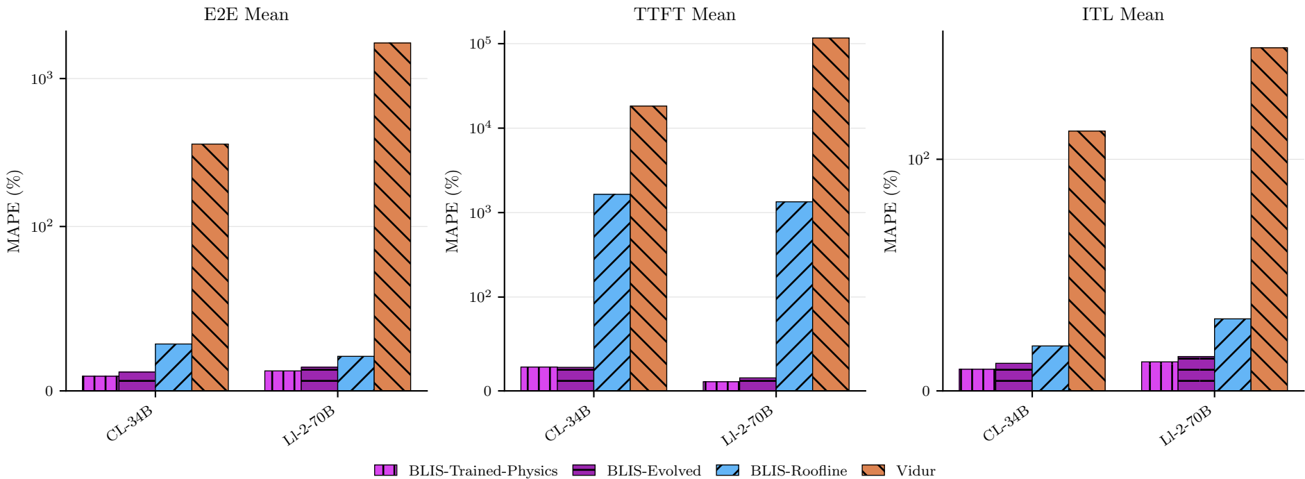
BLIS-Roofline & BLIS-Trained-Physics & BLIS-Evolved vs Vidur (n=4) ↓
